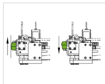
Installation situation independent of operating direction: Nozzle can be rotated 180°
