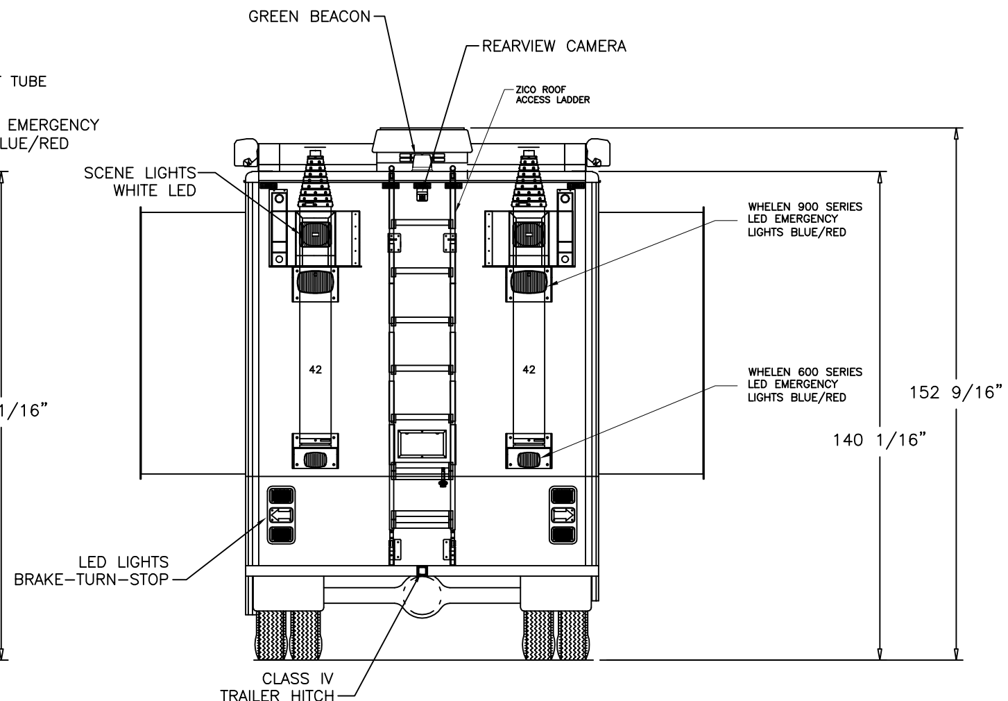
REAR ELEVATION
