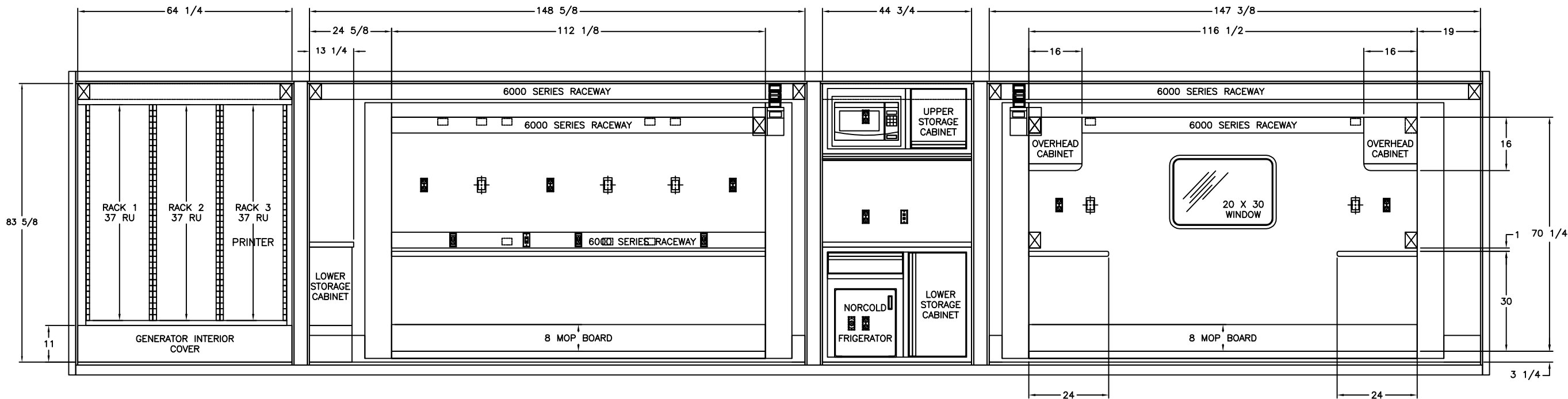
DRIVERS SIDE INTERIOR LAYOUT
