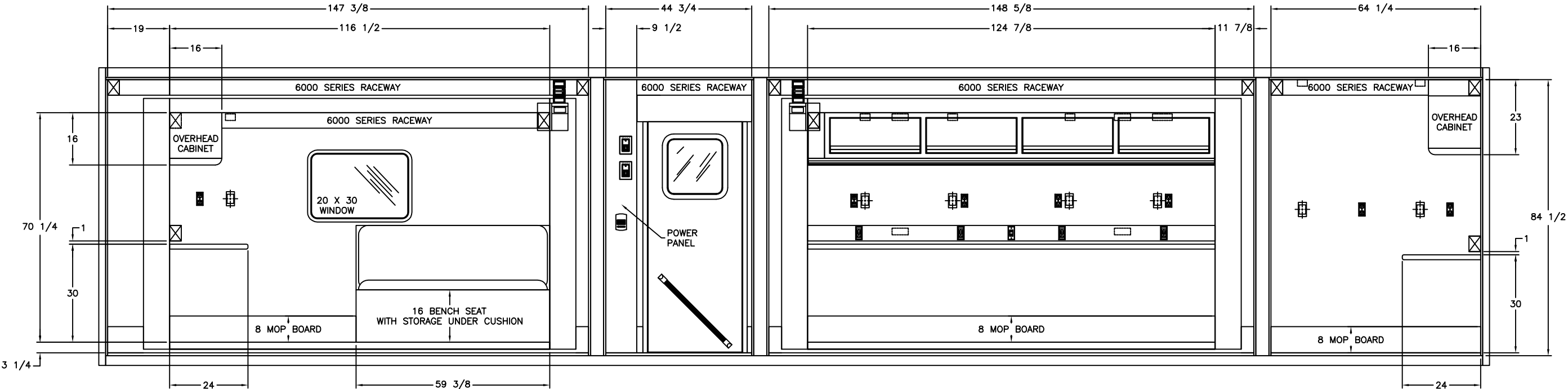
PASSENGERS SIDE INTERIOR LAYOUT
