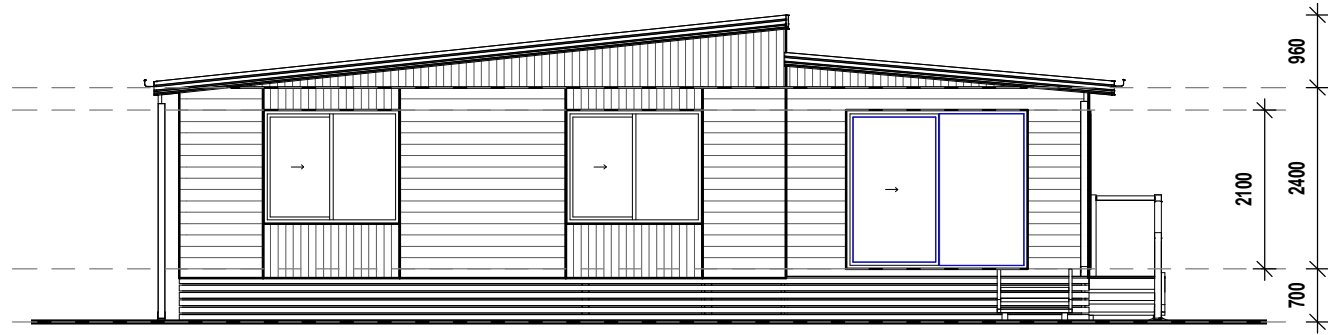
NORTHERN ELEVATION
