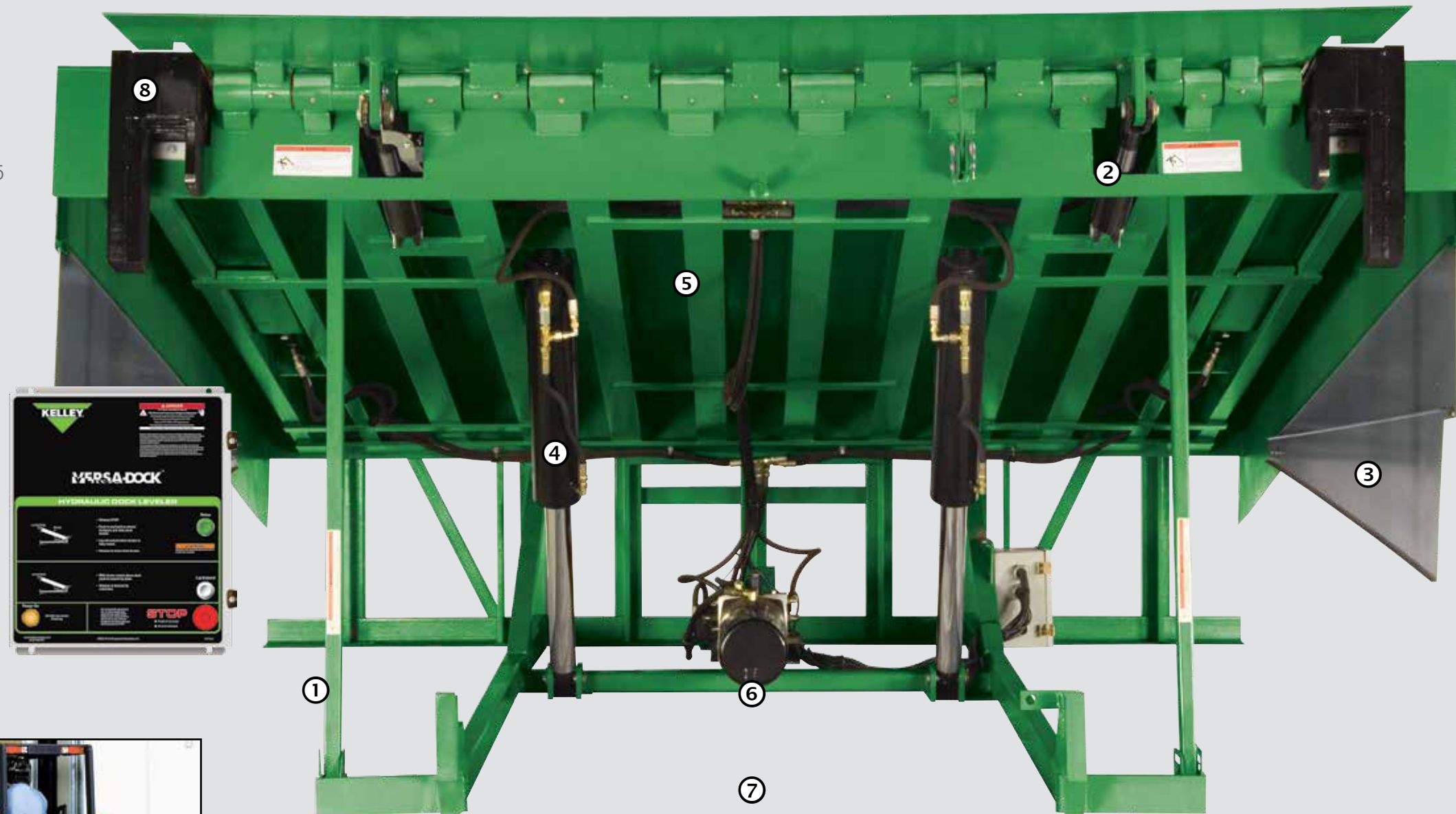
The VERSADOCK control panel features individual controls for all leveler functions and includes a mushroom-style stop for increased safety.
