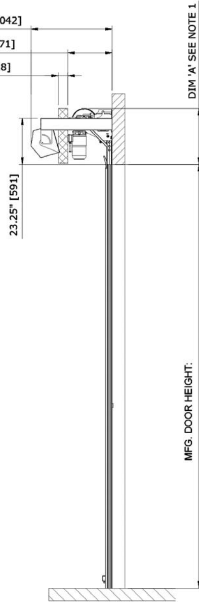
RIGHT VIEW
