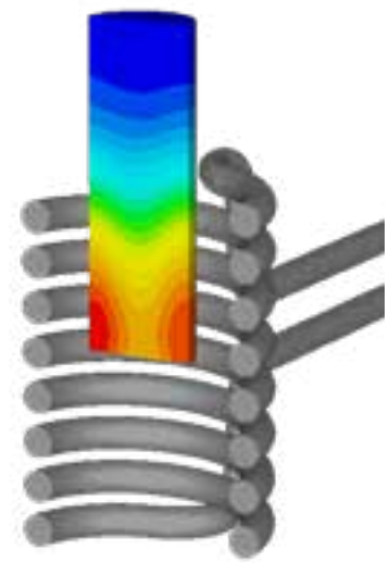
Temperature of the billet during induction heating
