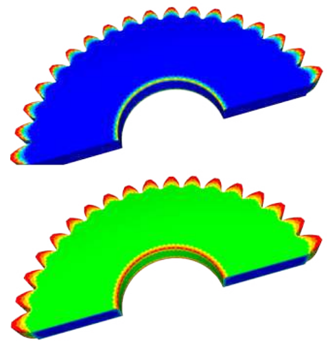
Predicting martensite and hardness
