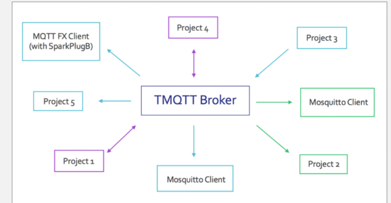
GATEWAY & CONNECTED TO RUNTIME PROJECT
