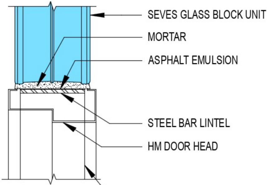
SECTION/ELEV
