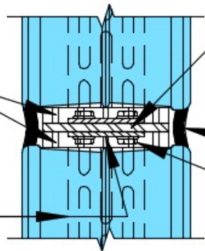
PLAN (JOINT ABOVE JAMB)
