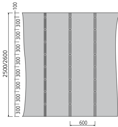
Application: Stud frame distance 600 mm from 20 mm. Dimensions: 2500 x 600 mm and 2500 x 1200 mm
