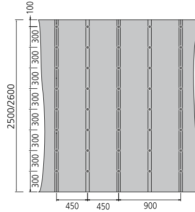
Application: Stud frame distance for max. 450 mm for building boards from 10 mm. Dimensions: 2500 x 900 mm
