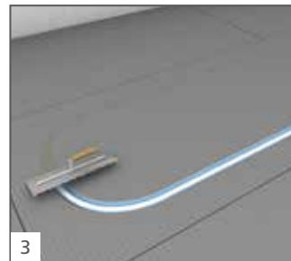
3 Install tubing into the groove. Fill tile adhesive into the pipe duct.
