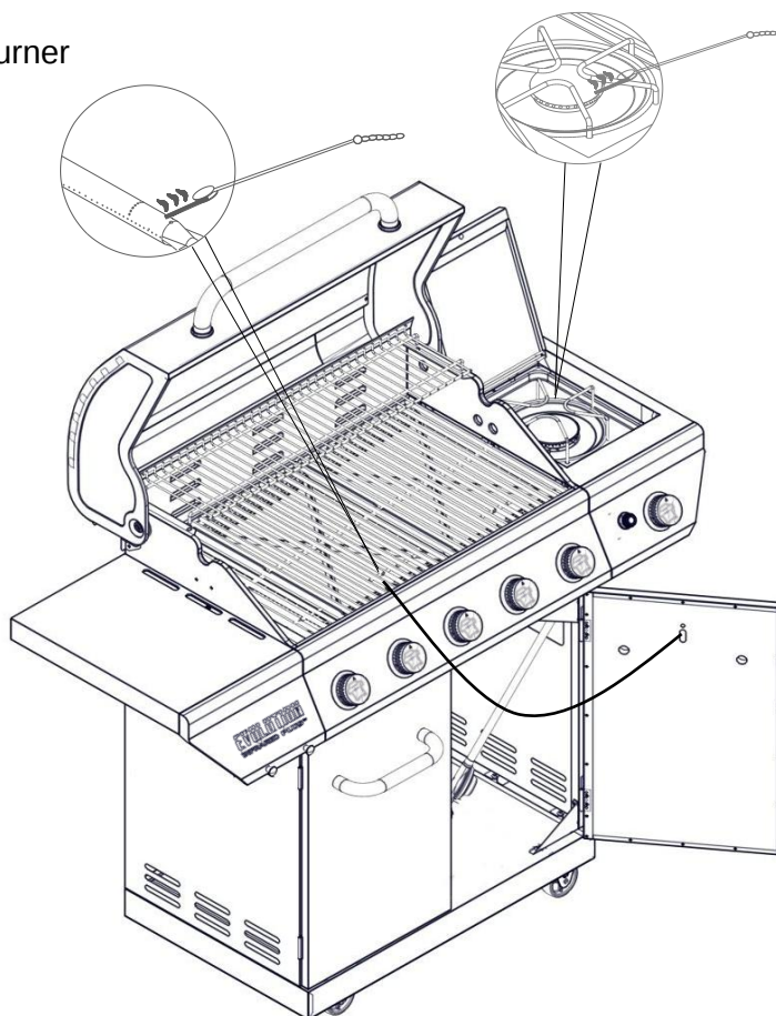
Side burner
