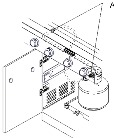
A. Gas pressure regulator/Hose assembly
