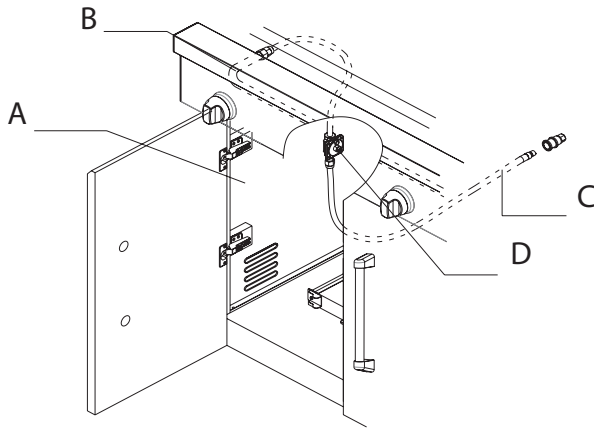
A. Left side panel B. Manifold C. 10 ft. (3.0 m) PVC gas hose D. Natural gas pressure regulator/hose assembly
