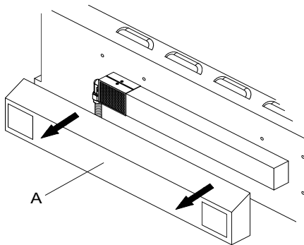
A. Access cover
