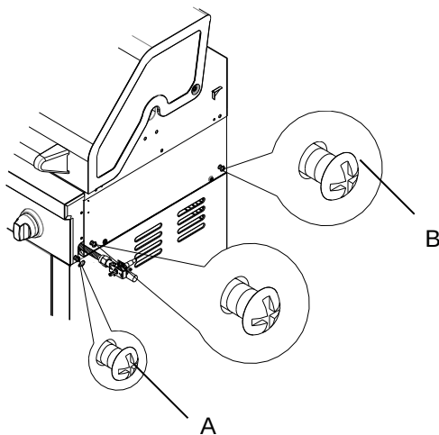
A. Grill control panel screws B. Grill side panel screws
