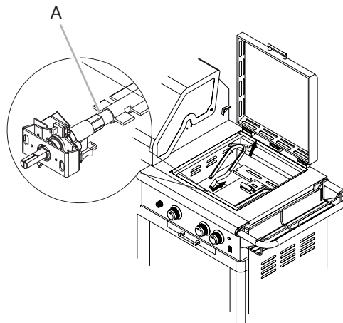
A. Burner/Orifice connection
