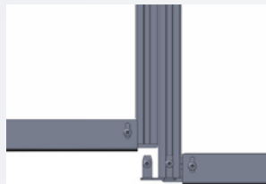
Secured Panelling Panels are secured at the top and the bottom by inserting the 4-finger bracket into the frame channel.
