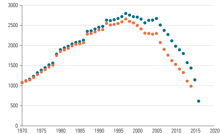
Figure 9: The number of species (above) and populations (below) contributing to the index in each year for both the 2018 (orange) and 2020 (blue) Living Planet Report. WWF/ZSL (2020) 22 .
