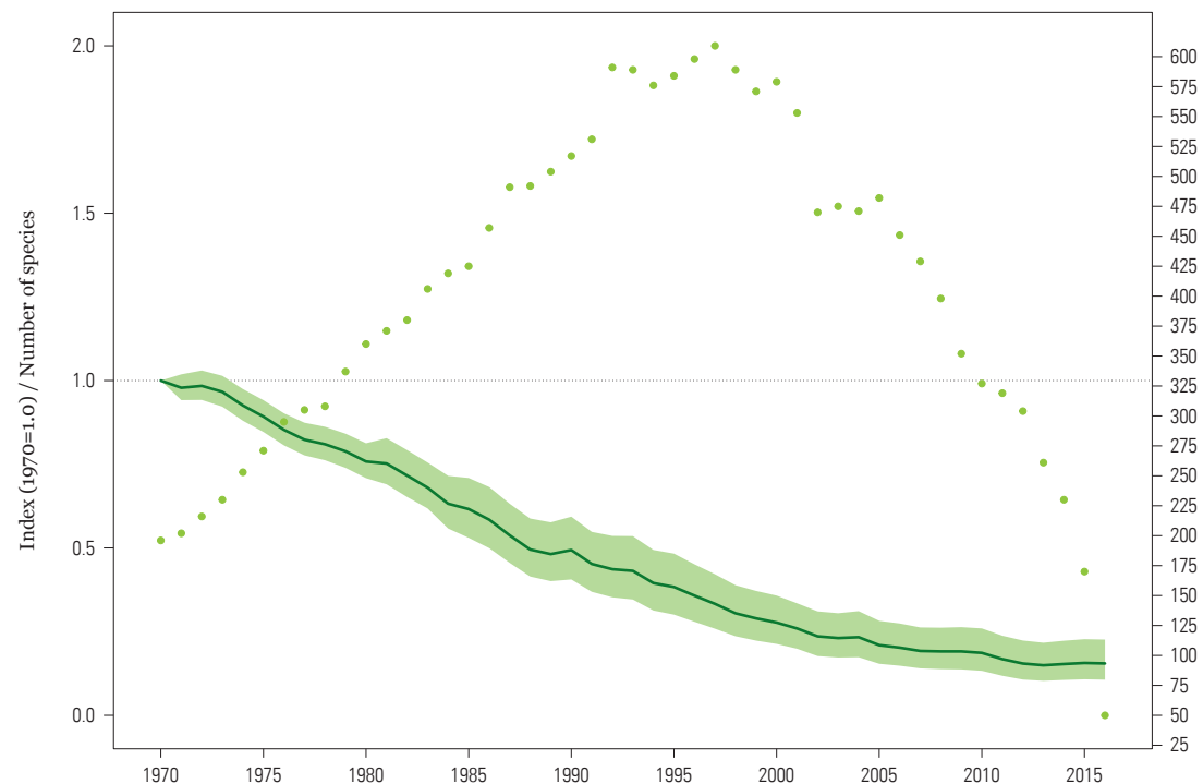
Figure 3: Index of abundance for 944 freshwater vertebrate species (final index value = -84%; range = -77% to -89%) monitored between 1970 and 2016, and the number of species contributing to the index in each year (pale green dots). WWF/ZSL (2020) 22 .
