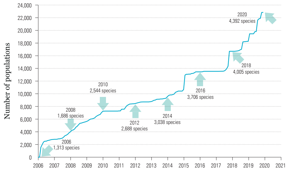
Figure 10: The cumulative number of population time-series in the LPI database and number of species in each Living Planet Report since 2006. WWF/ZSL (2020) 22 .
