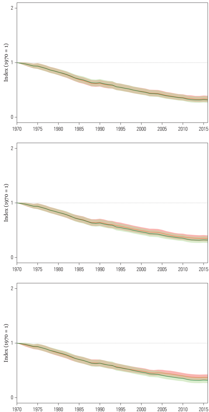
Figure 8: Indices of abundance for vertebrate species monitored between 1970 and 2016, calculated excluding time-series with data covering less than 3 years (top, 19,470 populations of 4,094 species), 5 years (middle, 16,579 populations for 3,760) and 10 years (bottom, 12,180 populations of 3,179 species). The global LPI trend is provided for comparison (in green). WWF/ZSL (2020) 22 .
