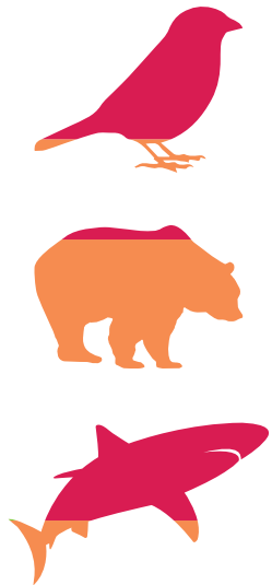
Figure 4: An illustration of how the average percentage change of the trend differs from the change in total number of animals lost (in percentage). WWF/ZSL (2020) 22 .
