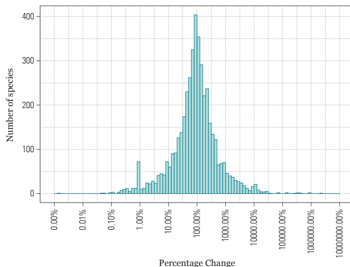
Figure 6: Histogram of the total change between 1970 and 2016 of the 4,392 species contributing to the global LPI Species are binned based on the magnitude of the total change they go through during the entirety of the time-series (one or more) they are represented by in the dataset. : “100%” is the size of the species population at the beginning of the time-series, so the frequency at “100%” represents time series with no change in population size (stable population). The remaining percentages reflect how many times larger or smaller the species populations are compared to the beginning of the time series. WWF/ZSL (2020) 28 .
