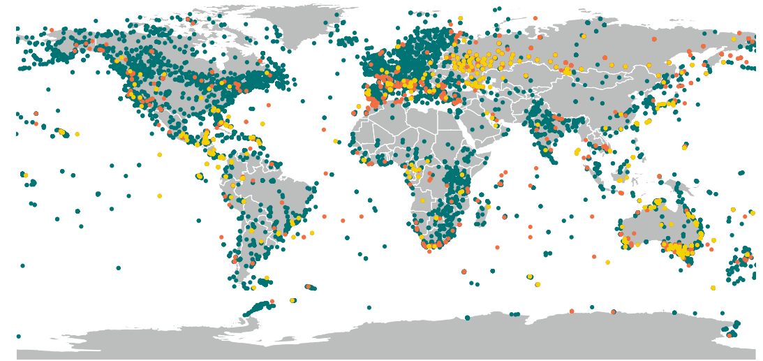
Figure 12: Map showing the locations of the populations in the LPI monitored in specific locations. Newly added populations since the last report are highlighted in orange, or in red for species new to the LPI. WWF/ZSL (2020) 22 .
