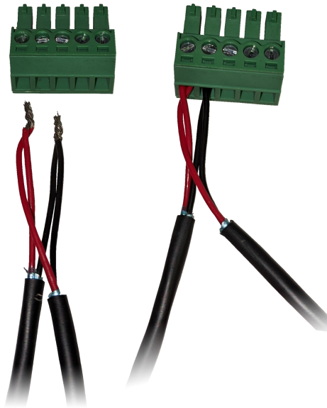
RS-485 Home-Run connection
