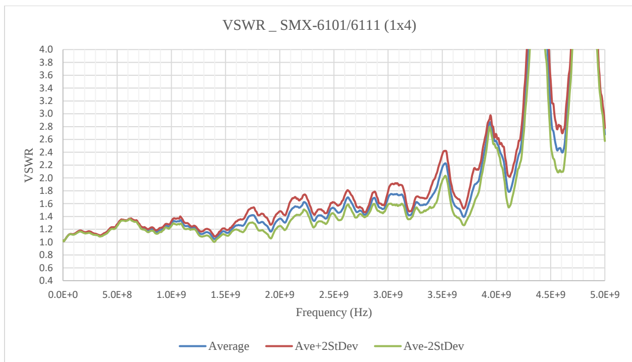
FIGURE 3-82: SMX-6101 SMB VSWR GRAPH
