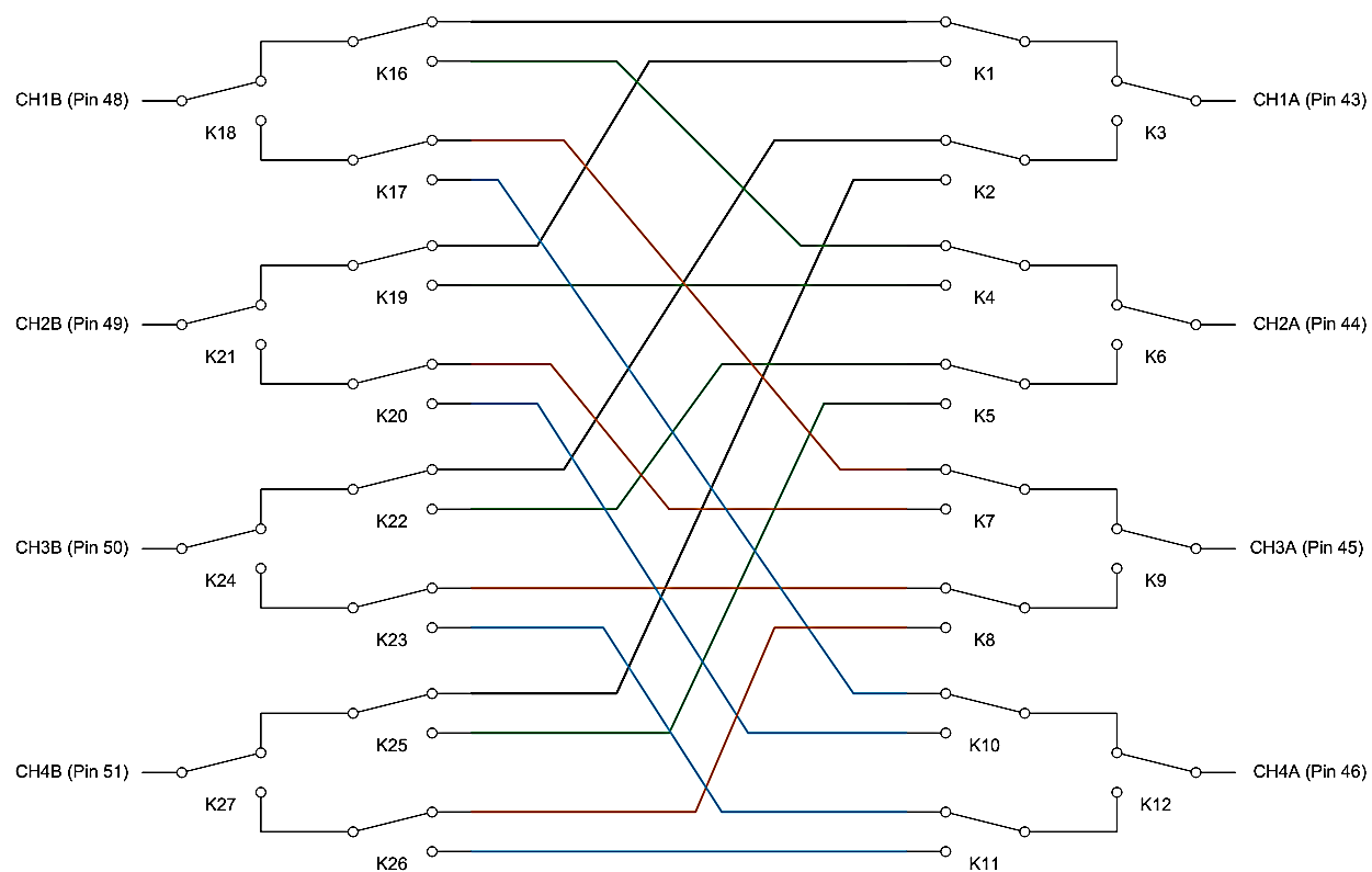
FIGURE 3-114: SMX-6144 PkZ LOGICAL DIAGRAM
