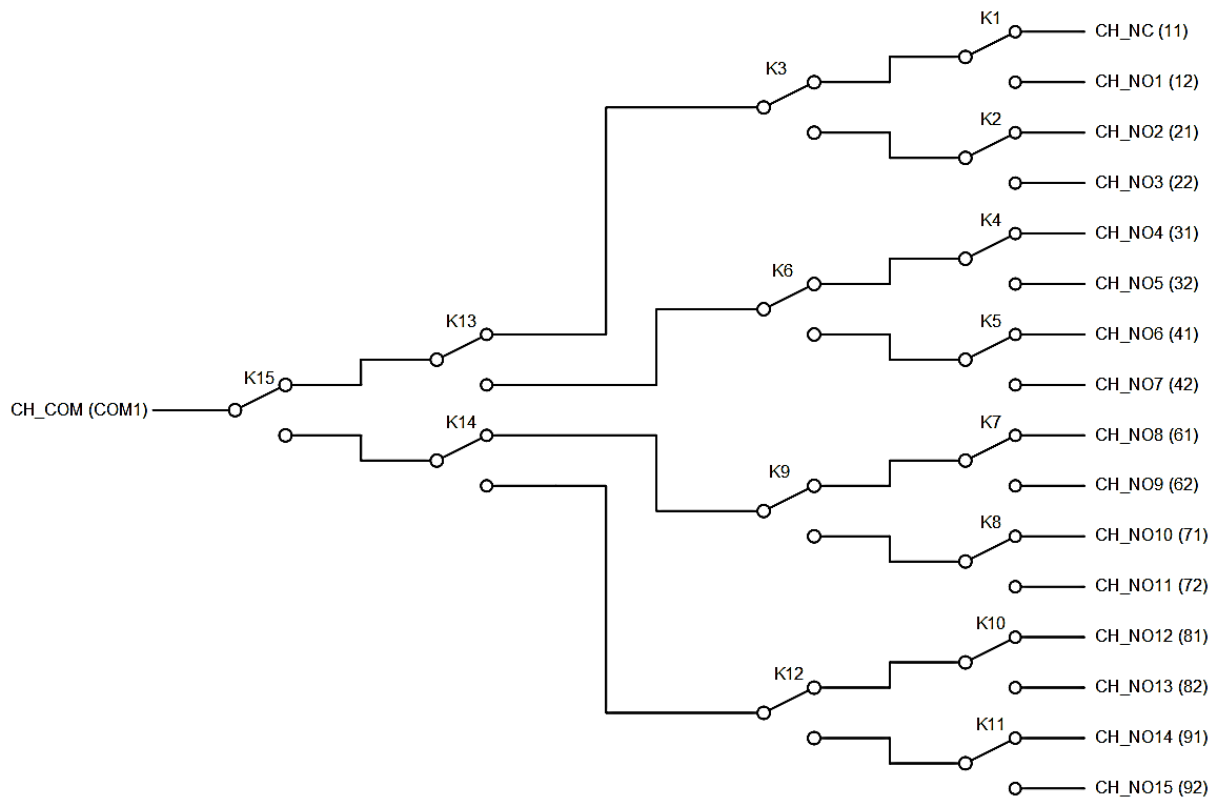
FIGURE 3-95: SMX-6116 SMB LOGICAL DIAGRAM
