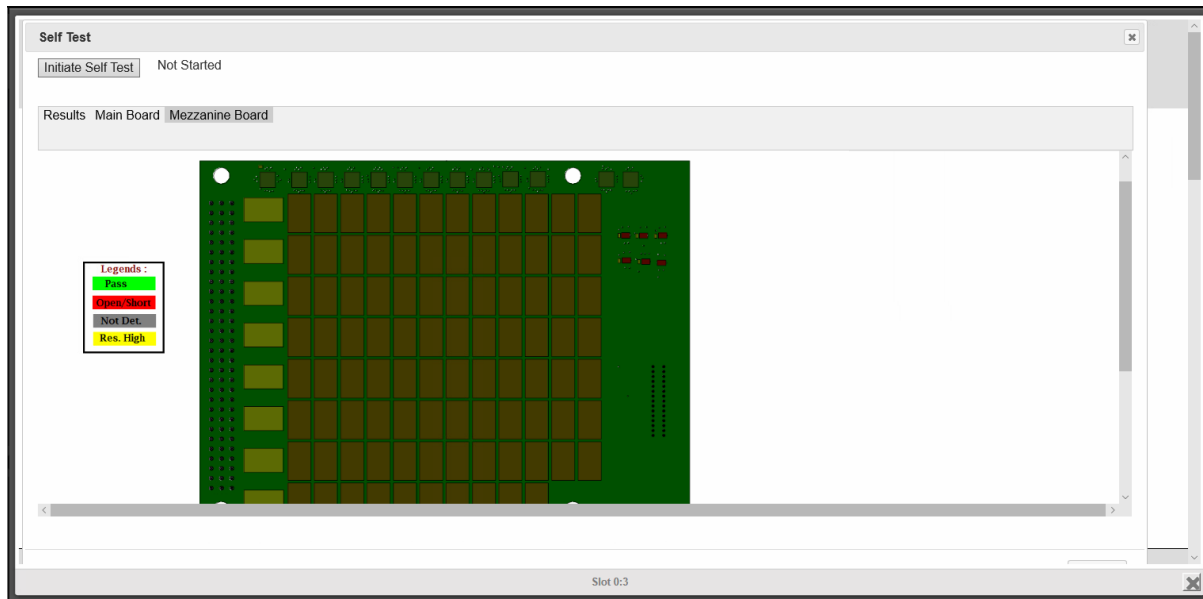
FIGURE 3-55: SMX-4410 SELFTEST-MEZZANINE BOARD RELAY LOCATION PAGE
