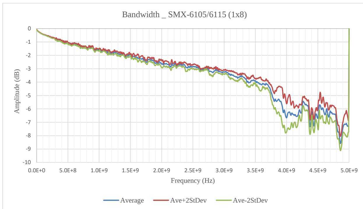
FIGURE 3-101: SMX-6105 SMB BANDWIDTH GRAPH
