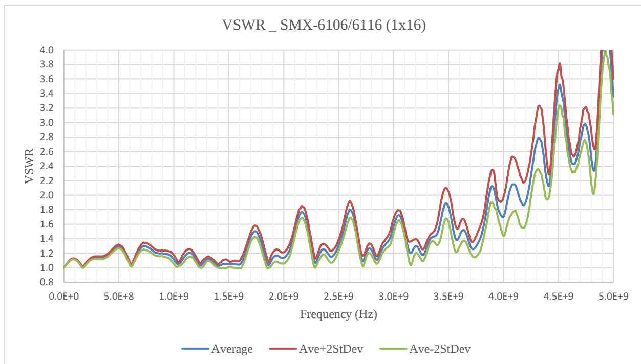
FIGURE 3-92: SMX-6106 SMB VSWR GRAPH
