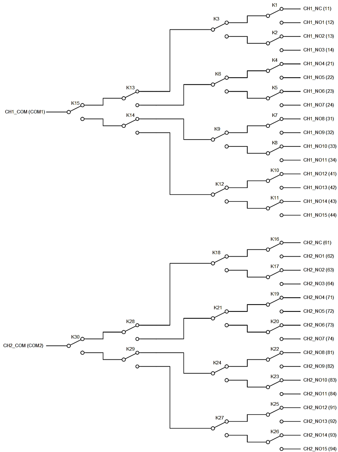
FIGURE 3-90: SMX-6106 SMB LOGICAL DIAGRAM
