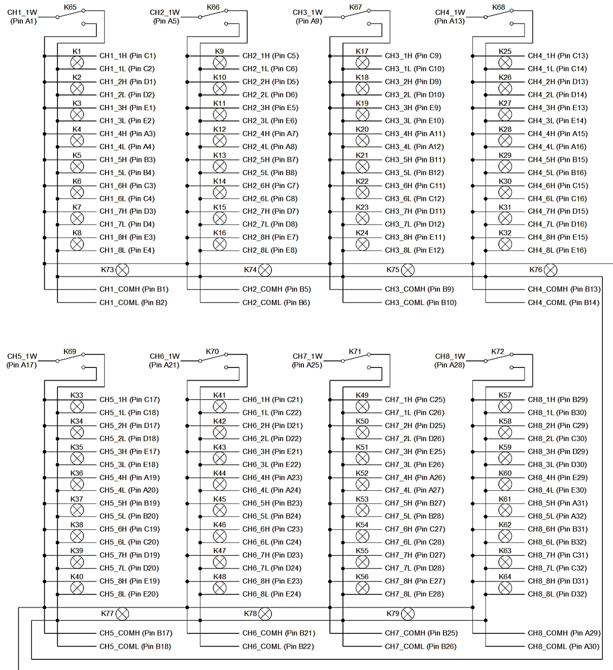
FIGURE 3-5: SMX-3001 LOGICAL DIAGRAM
