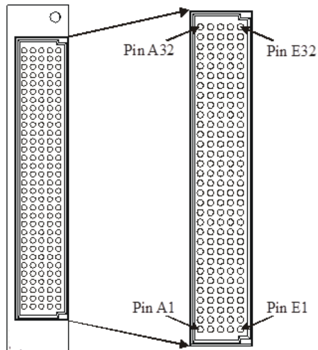
FIGURE 3-11: SMX-3002DS FRONT PANEL (FRONT VIEW)
