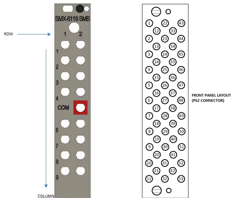
FIGURE 3-93: SMX-6116 FRONT PANEL LAYOUT(SMB CONNECTOR -LEFT IMAGE, PkZ CONNECTOR- RIGHT IMAGE)
