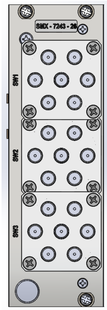
FIGURE 3-123: SMX-7243-26 FRONT PANEL
