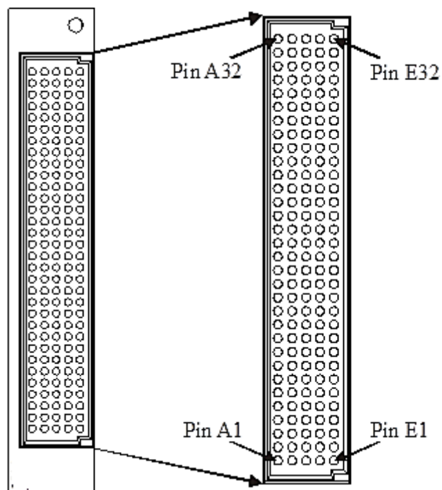
FIGURE 3-27: SMX-3007 FRONT PANEL CONNECTOR PINS (FRONT VIEW)
