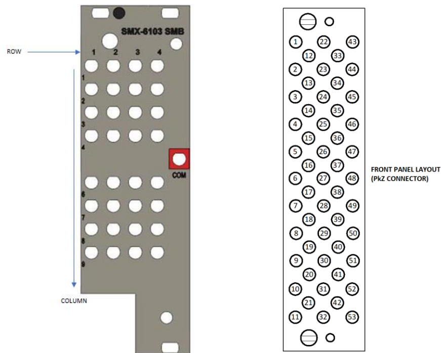
FIGURE 3-108: SMX-6103 FRONT PANEL LAYOUT(SMB CONNECTOR -LEFT IMAGE, PkZ CONNECTOR- RIGHT IMAGE)
