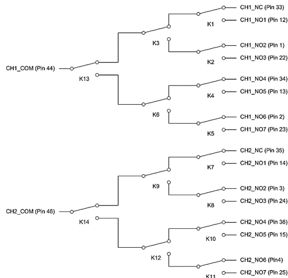
FIGURE 3-104: SMX-6115 PkZ LOGICAL DIAGRAM
