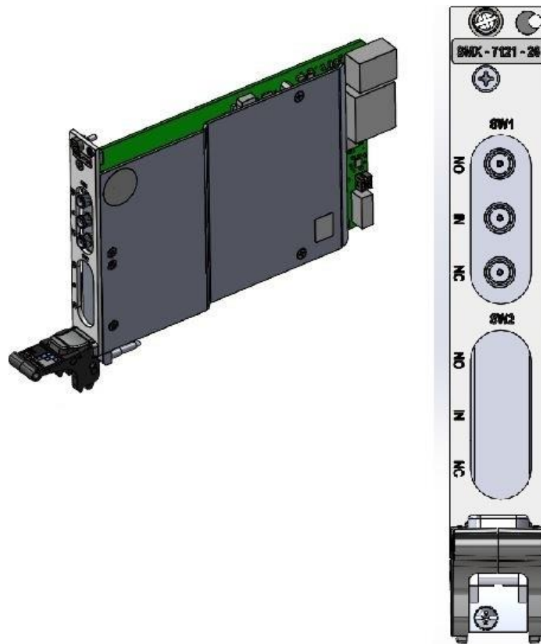
FIGURE 3-118: SMX-7121-26 FRONT PANEL (ISOMETRIC AND FRONT VIEWS)
