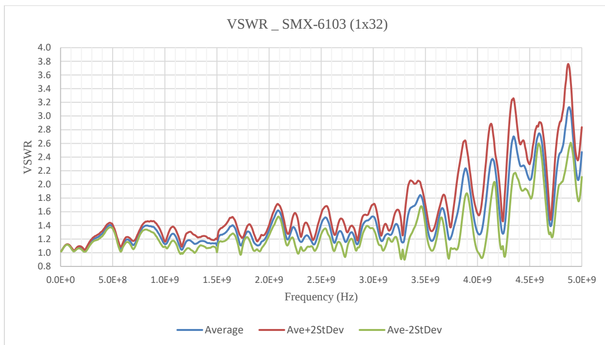
FIGURE 3-112: SMX-6103 SMB VSWR GRAPH
