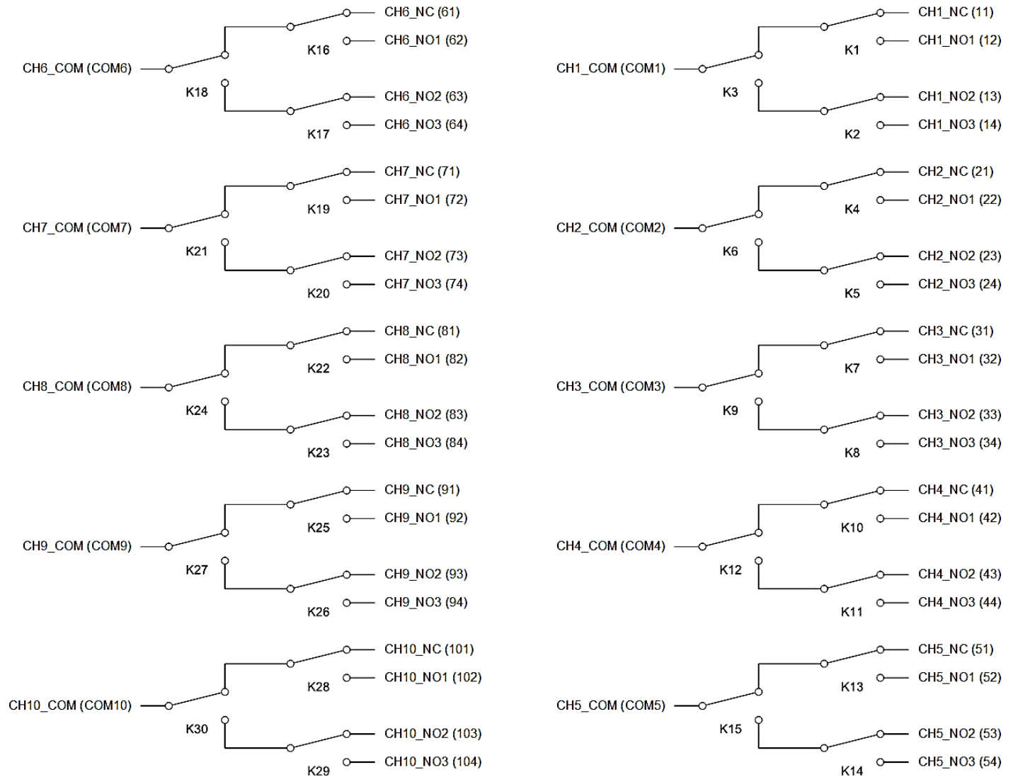
FIGURE 3-80: SMX-6101 SMB LOGICAL DIAGRAM
