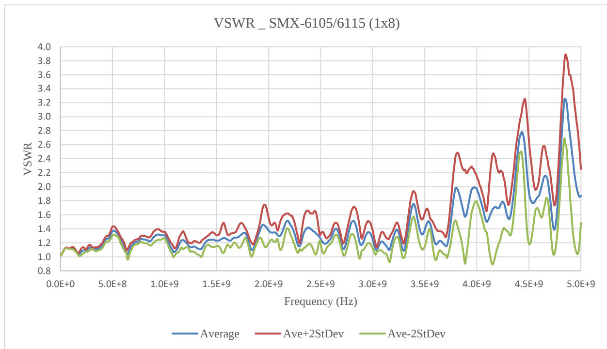
FIGURE 3-107: SMX-6115 SMB VSWR GRAPH
