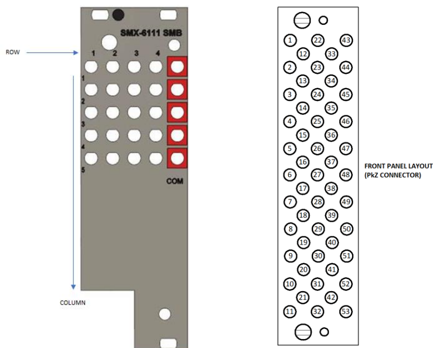
FIGURE 3-83: SMX-6111 FRONT PANEL LAYOUT(SMB CONNECTOR -LEFT IMAGE, PkZ CONNECTOR- RIGHT IMAGE)
