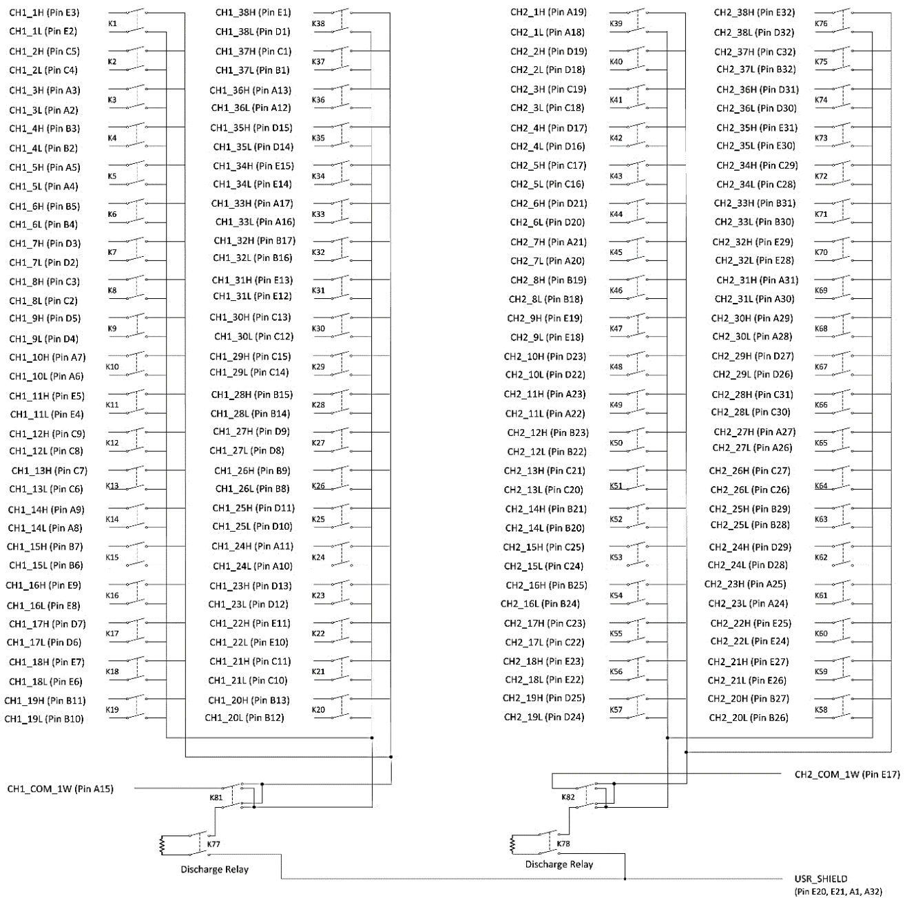
FIGURE 3-36: SMX-3277DS LOGICAL DIAGRAM
