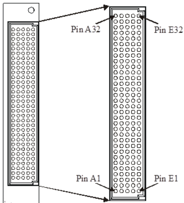
FIGURE 3-35: SMX-3277DS FRONT PANEL CONNECTOR (FRONT VIEW)
