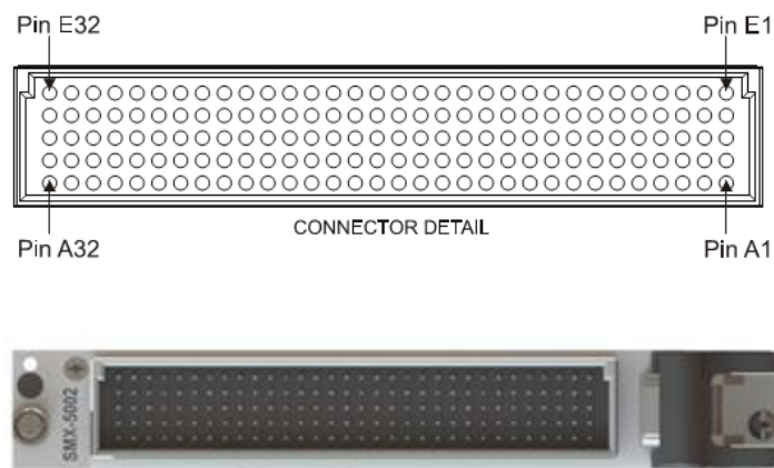
FIGURE 3-75: SMX-5002 CONNECTOR PIN LOCATIONS
