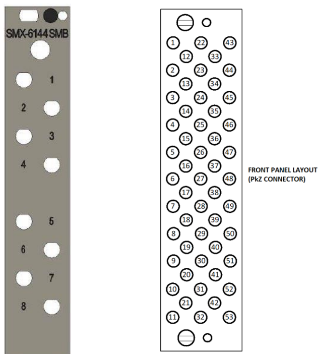
FIGURE 3-113: SMX-6144 FRONT PANEL LAYOUT(SMB CONNECTOR -LEFT IMAGE, PkZ CONNECTOR- RIGHT IMAGE)
