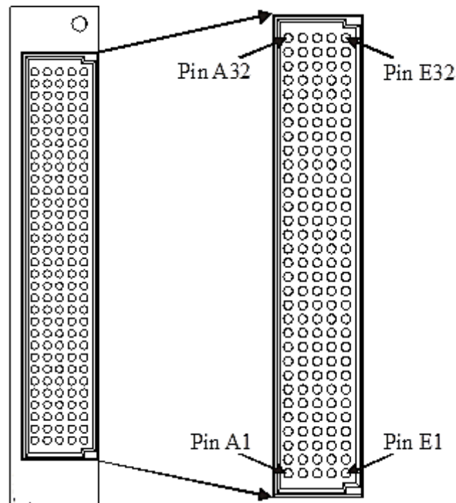
FIGURE 3-29: SMX-3276 FRONT PANEL CONNECTOR (FRONT VIEW)
