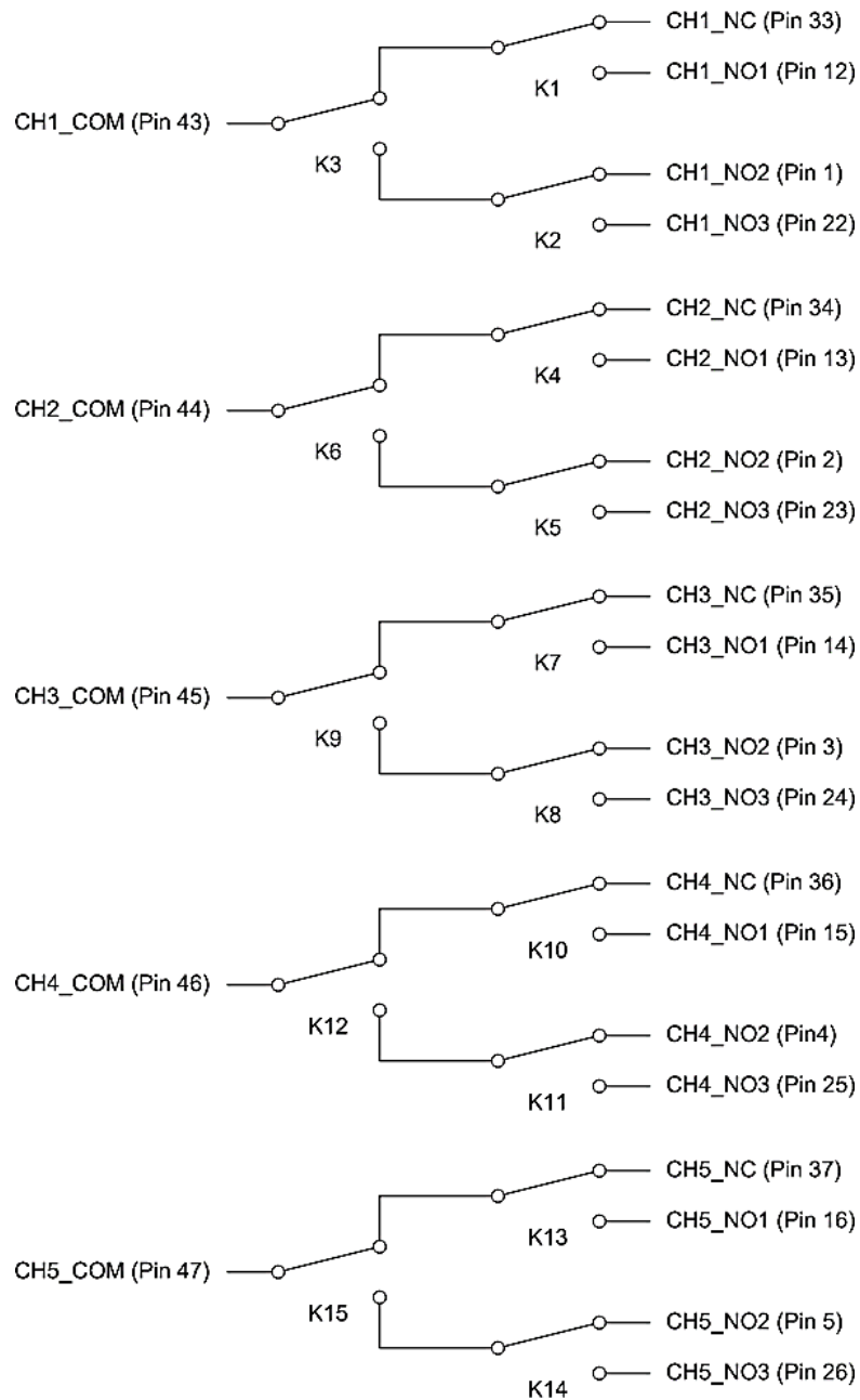
FIGURE 3-84: SMX-6111 PkZ LOGICAL DIAGRAM
