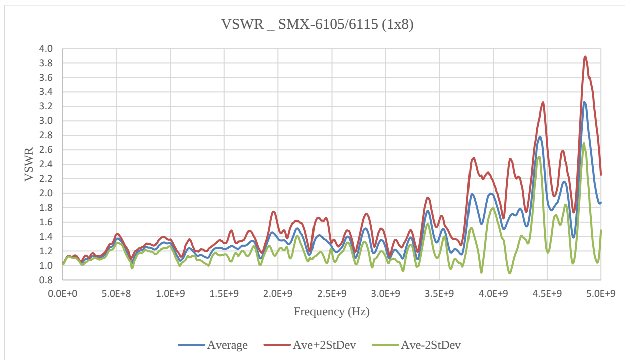
FIGURE 3-102: SMX-6105 SMB VSWR GRAPH
