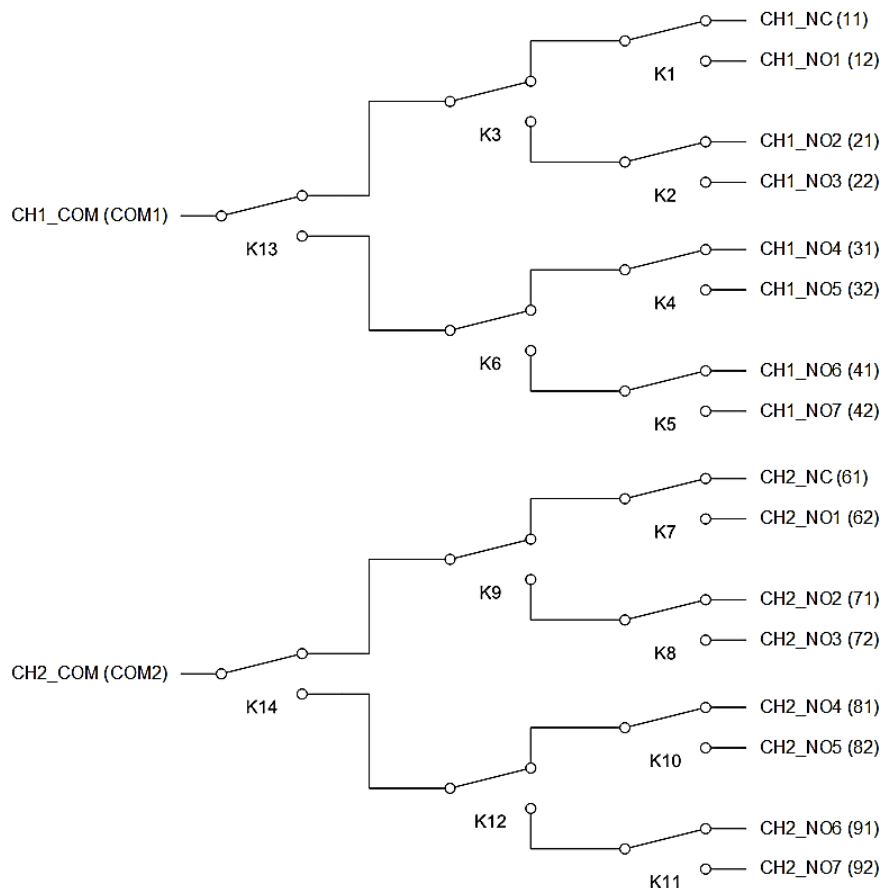
FIGURE 3-105: SMX-6115 SMB LOGICAL DIAGRAM
