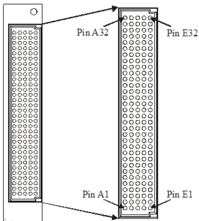
FIGURE 3-43: SMX-3279DS FRONT PANEL CONNECTOR (FRONT VIEW)
