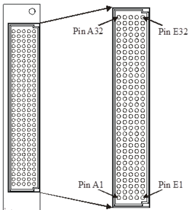
FIGURE 3-41: SMX-3279 FRONT PANEL CONNECTOR (FRONT VIEW)
