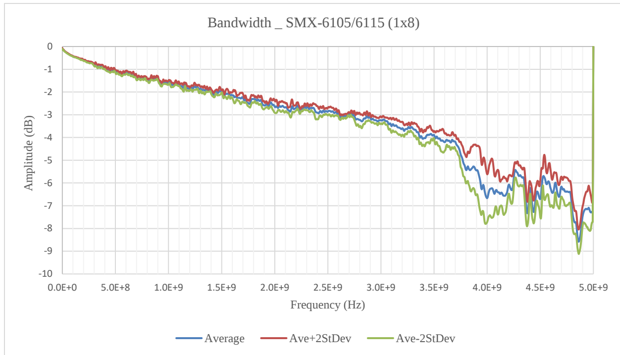
FIGURE 3-106: SMX-6115 SMB BANDWIDTH GRAPH
