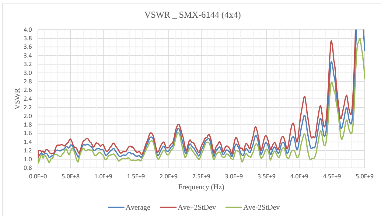
FIGURE 3-117: SMX-6144 SMB VSWR GRAPH
