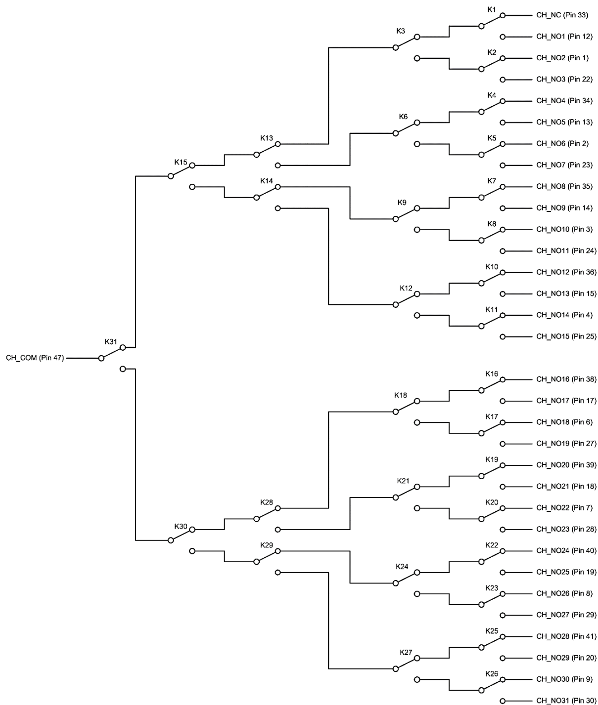
FIGURE 3-109: SMX-6103 PkZ LOGICAL DIAGRAM
