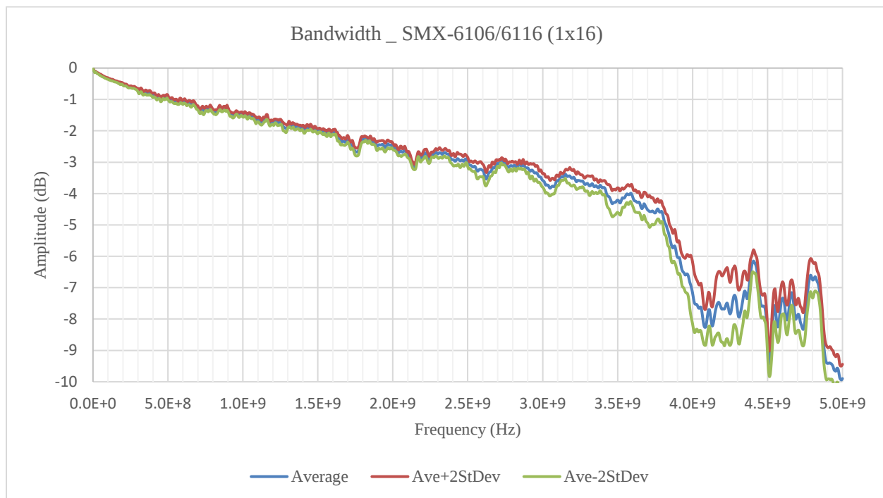
FIGURE 3-91: SMX-6106 SMB BANDWIDTH GRAPH
