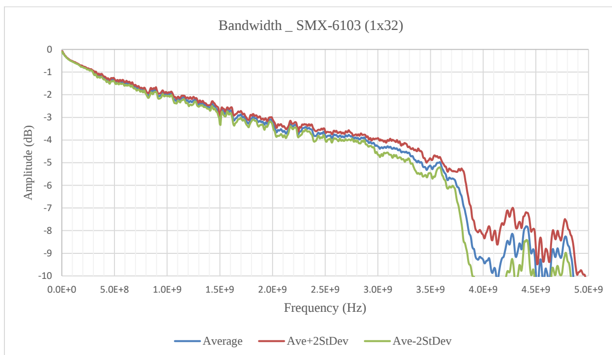
FIGURE 3-111: SMX-6103 SMB BANDWIDTH GRAPH
