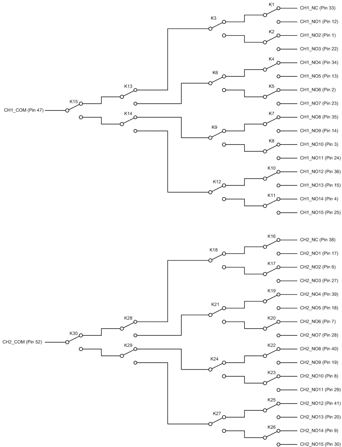
FIGURE 3-89: SMX-6106 PkZ LOGICAL DIAGRAM
