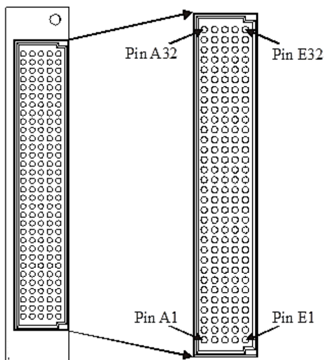
FIGURE 3-33: SMX-3277 FRONT PANEL CONNECTOR (FRONT VIEW)
