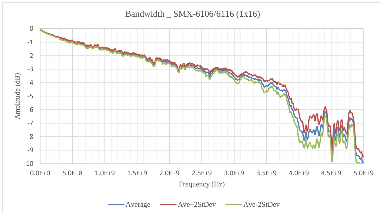
FIGURE 3-96: SMX-6116 SMB BANDWIDTH GRAPH
