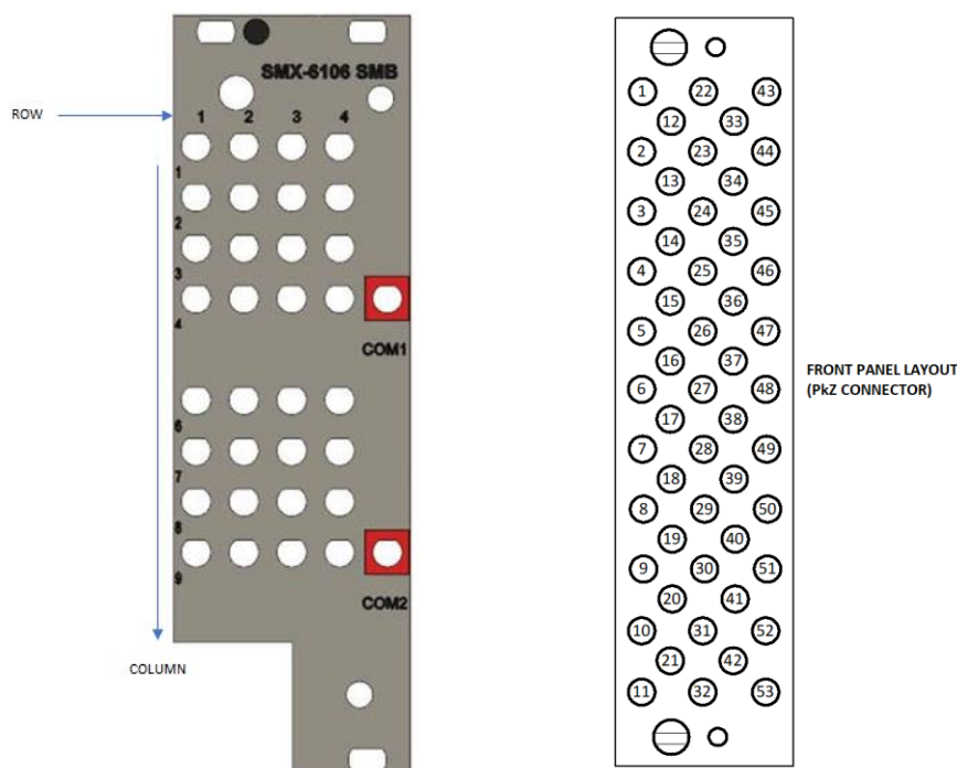
FIGURE 3-88: SMX-6106 FRONT PANEL LAYOUT(SMB CONNECTOR -LEFT IMAGE, PkZ CONNECTOR- RIGHT IMAGE)
