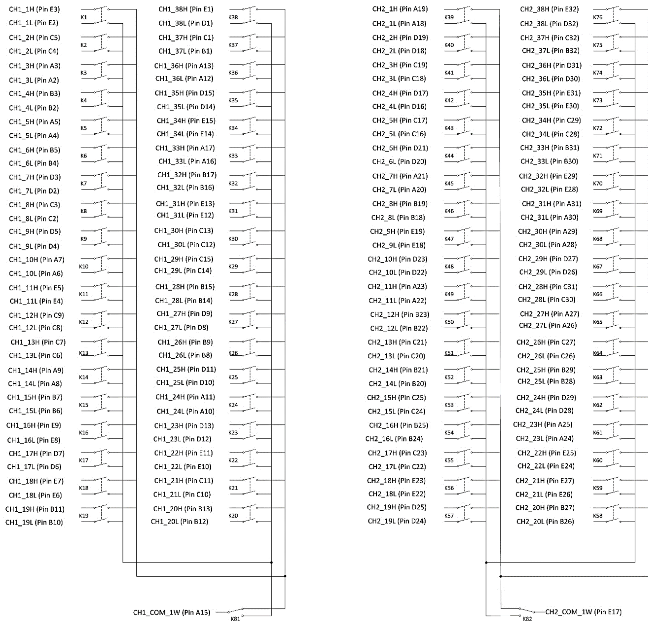
FIGURE 3-34: SMX-3277 LOGICAL DIAGRAM
