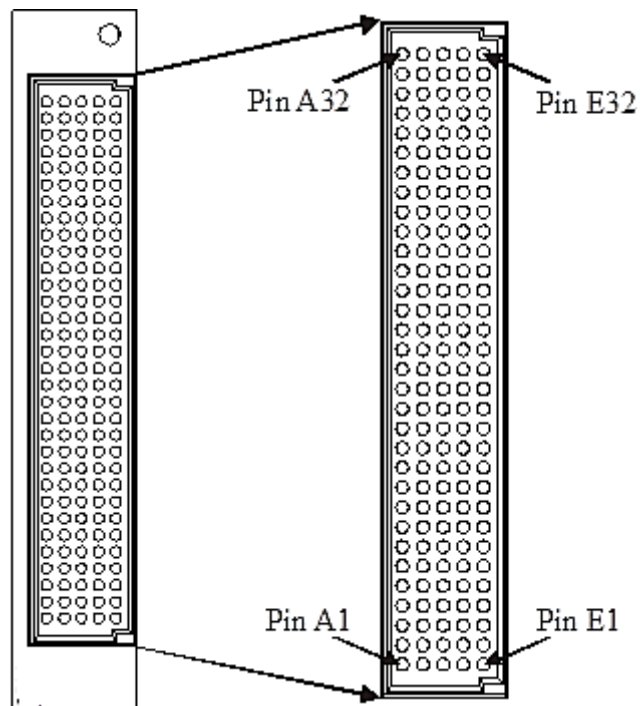
FIGURE 3-17: SMX-3004 FRONT PANEL CONNECTOR PINS (FRONT VIEW)
