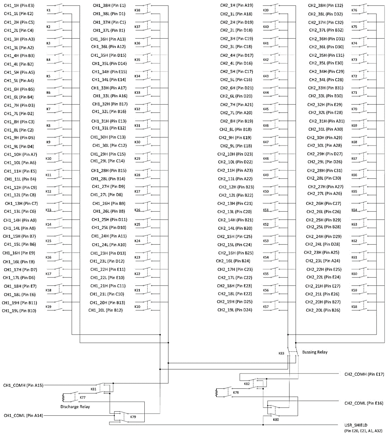
FIGURE 3-32: SMX-3276DS LOGICAL DIAGRAM
