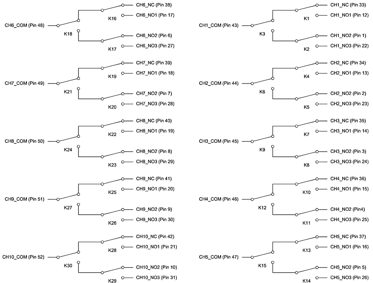
FIGURE 3-79: SMX-6101 PkZ LOGICAL DIAGRAM
