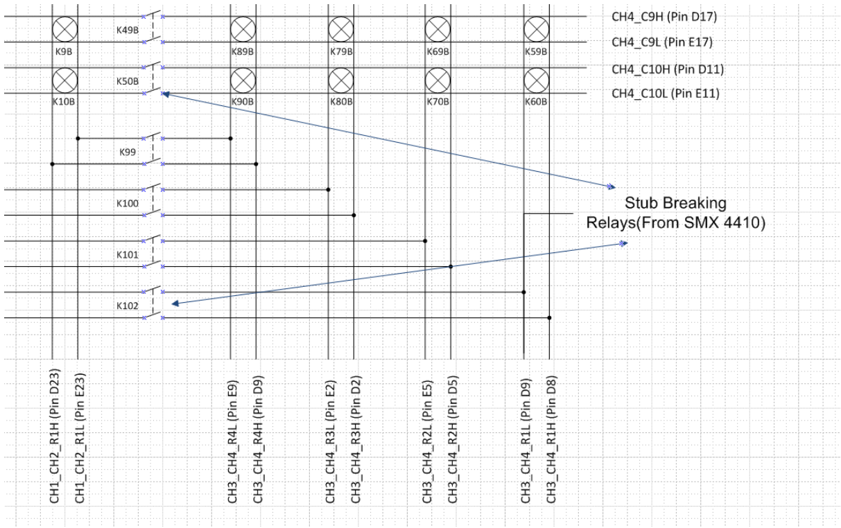
FIGURE 2-1: STUB BREAKING RELAYS
