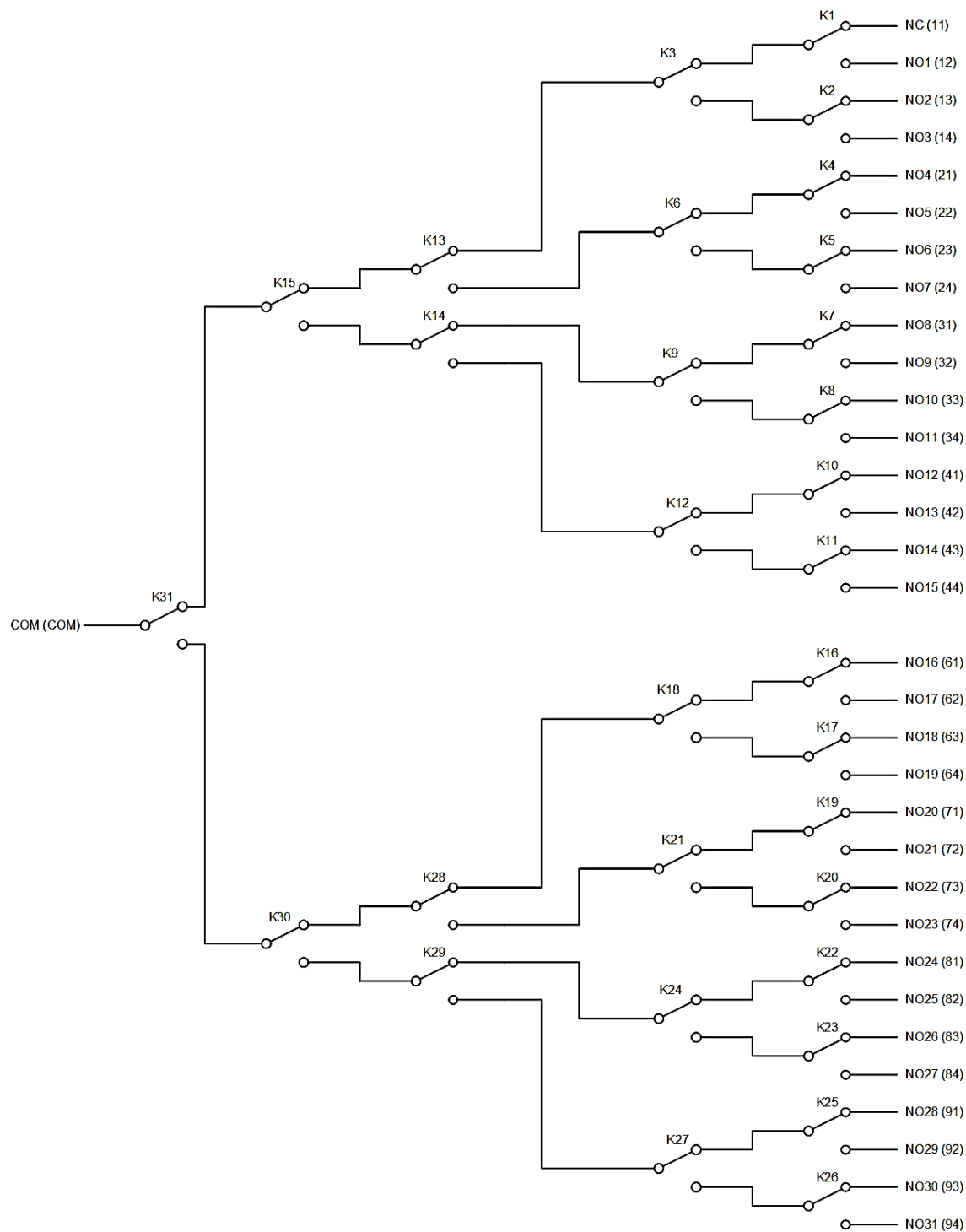
FIGURE 3-110: SMX-6103 SMB LOGICAL DIAGRAM
