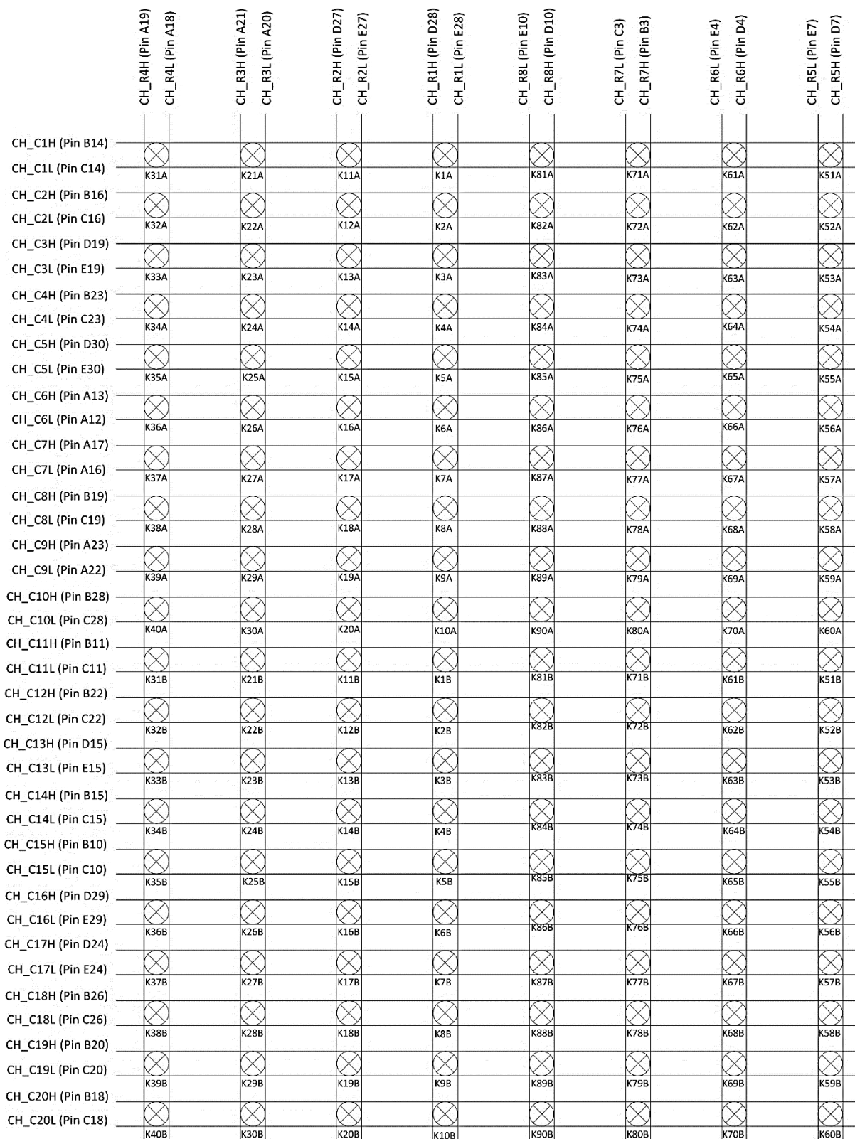
FIGURE 3-72: SMX-4415 LOGICAL DIAGRAM
