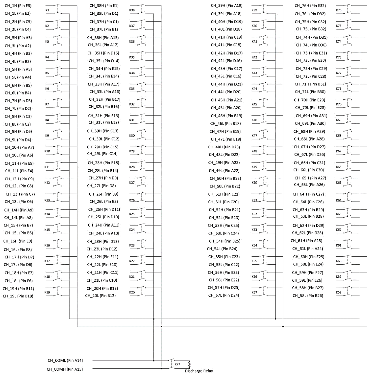
FIGURE 3-44: SMX-3279DS LOGICAL DIAGRAM
