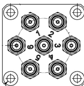
FIGURE 3-121: SMX-7241-26 SWITCH FRONT PANEL PORT ASSIGNMENT
