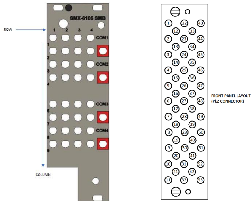
FIGURE 3-98: SMX-6105 FRONT PANEL LAYOUT(SMB CONNECTOR -LEFT IMAGE, PkZ CONNECTOR- RIGHT IMAGE)
