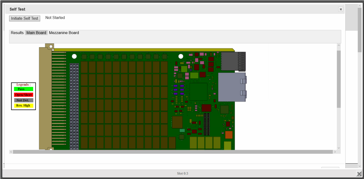
FIGURE 3-54: SMX-4410 SELFTEST-MAIN BOARD RELAY LOCATION PAGE
