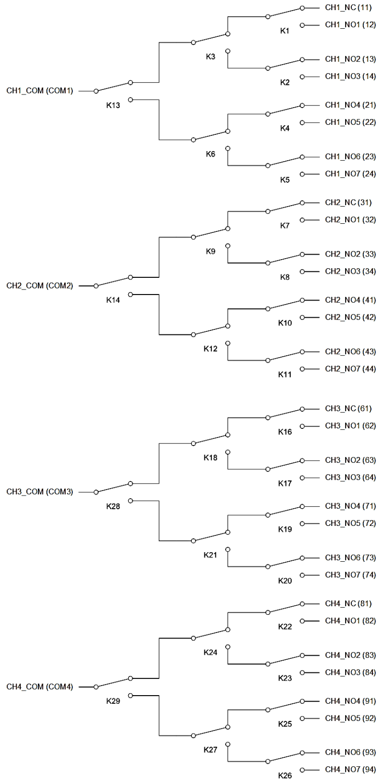
FIGURE 3-100: SMX-6105 SMB LOGICAL DIAGRAM
