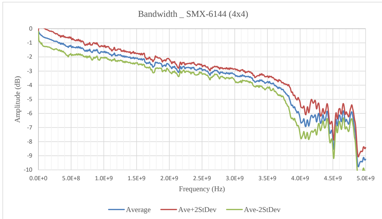
FIGURE 3-116: SMX-6144 SMB BANDWIDTH GRAPH
