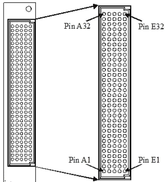
FIGURE 3-19: SMX-3004DS FRONT PANEL (FRONT VIEW)
