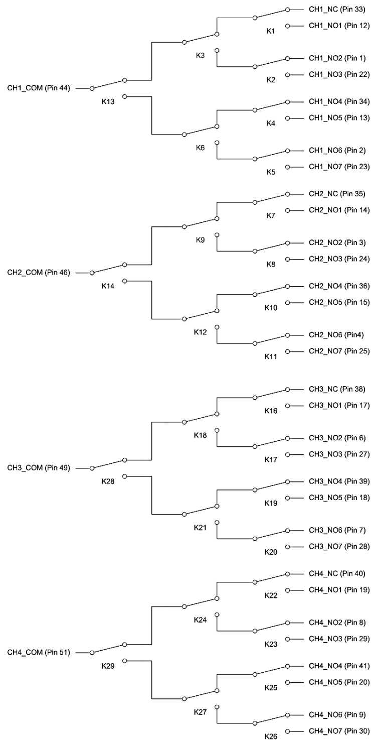
FIGURE 3-99: SMX-6105 PkZ LOGICAL DIAGRAM
