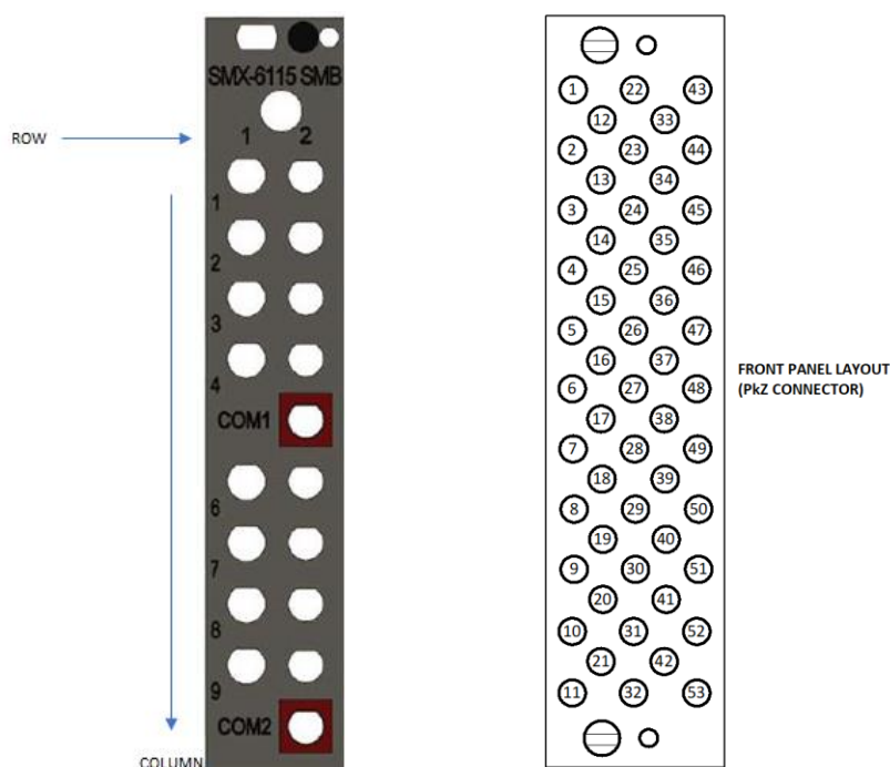
FIGURE 3-103: SMX-6115 FRONT PANEL LAYOUT(SMB CONNECTOR -LEFT IMAGE, PkZ CONNECTOR- RIGHT IMAGE)
