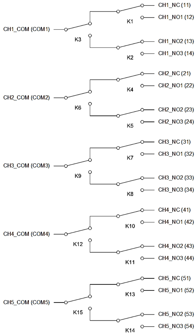
FIGURE 3-85: SMX-6111 SMB LOGICAL DIAGRAM
