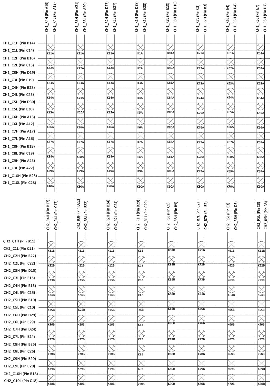
FIGURE 3-70: SMX-4414 LOGICAL DIAGRAM
