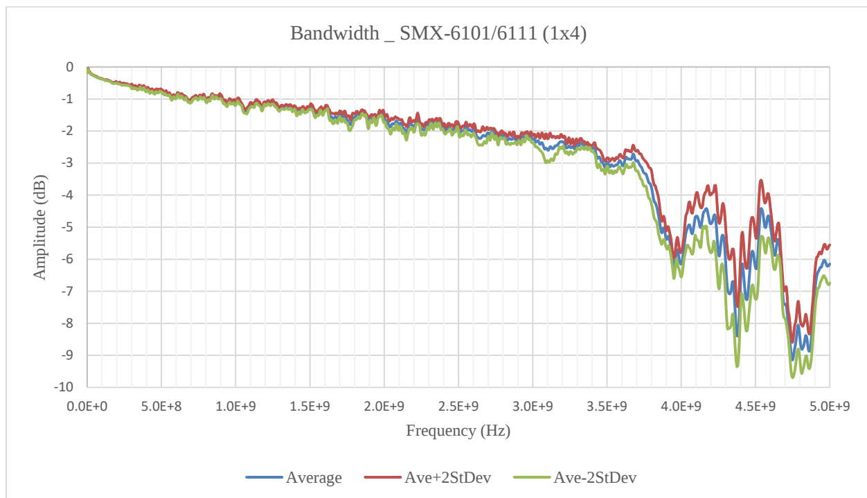
FIGURE 3-86: SMX-6111 SMB BANDWIDTH GRAPH
