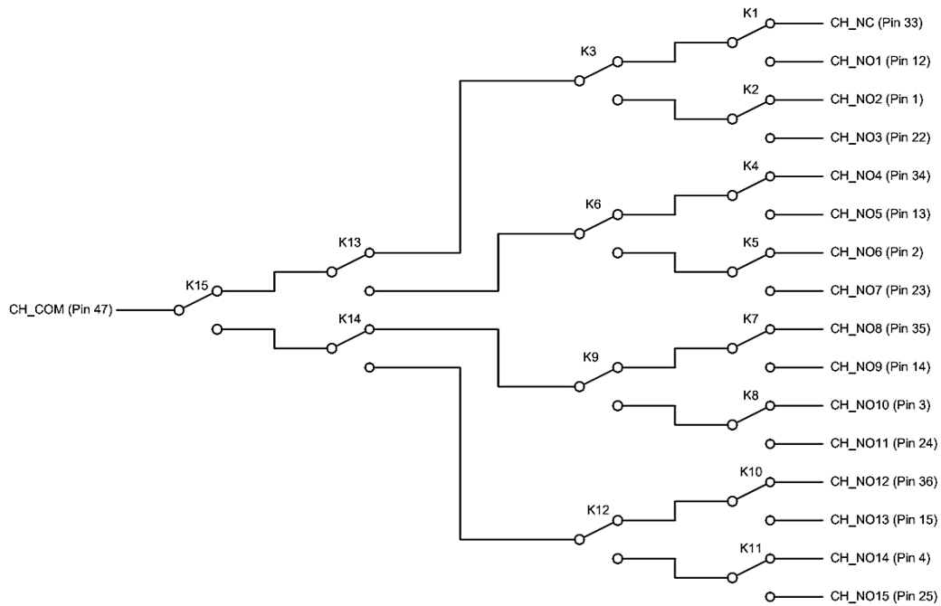
FIGURE 3-94: SMX-6116 PkZ LOGICAL DIAGRAM
