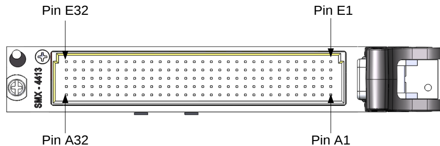
FIGURE 3-67: SMX-4413 FRONT PANEL (FRONT VIEW)
