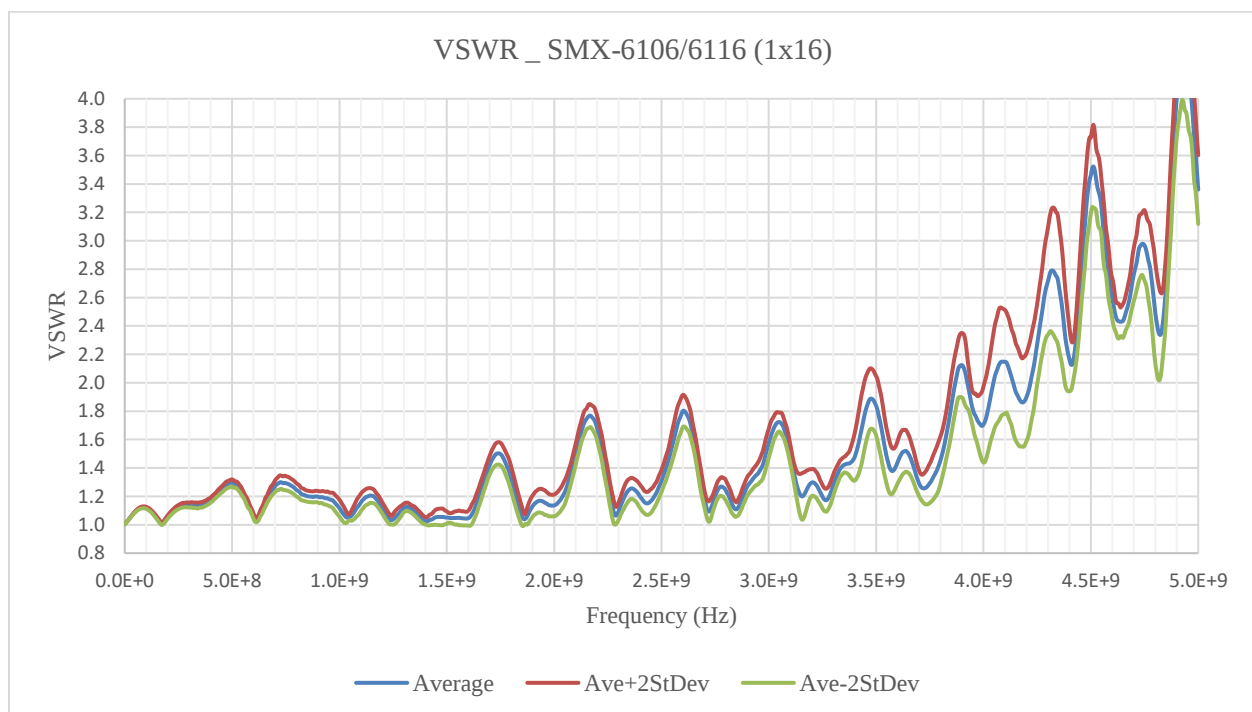
FIGURE 3-97: SMX-6116 SMB VSWR GRAPH
