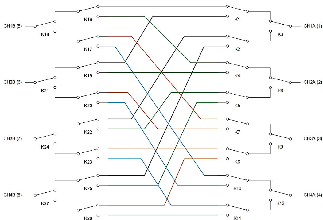
FIGURE 3-115: SMX-6144 SMB LOGICAL DIAGRAM
