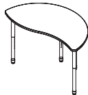
Nebula
