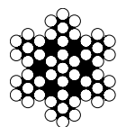
flexible wire construction
