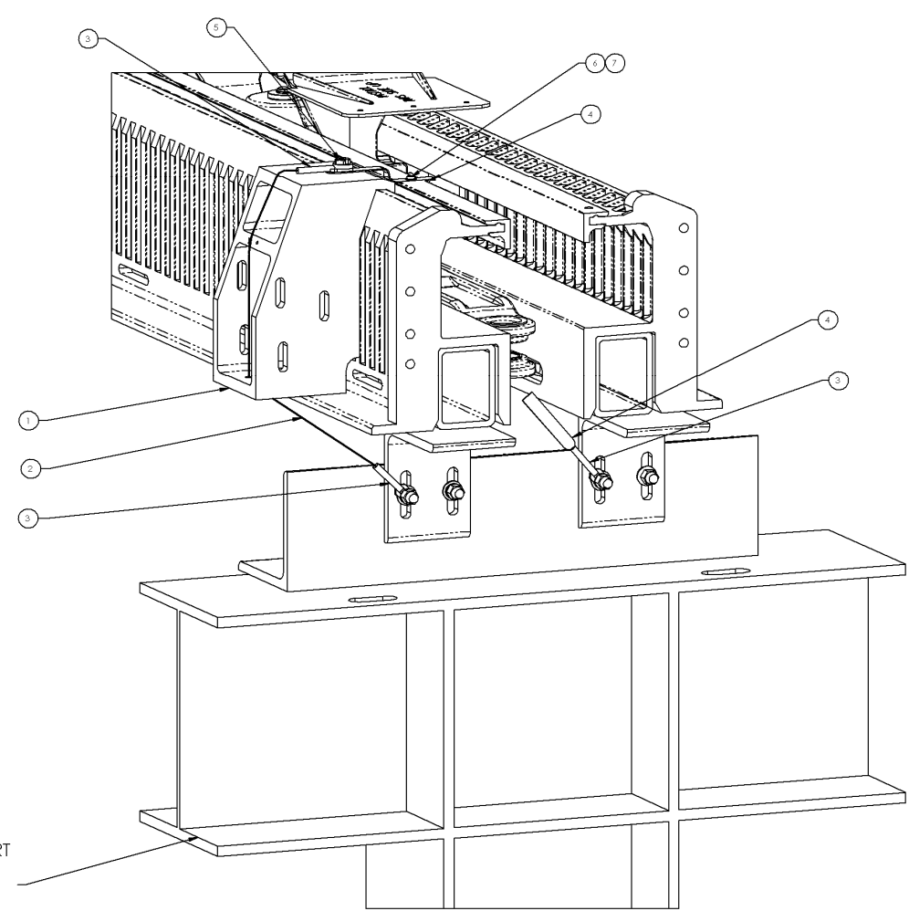
Figure 9-12 Static Dissipation Kit Assembly
