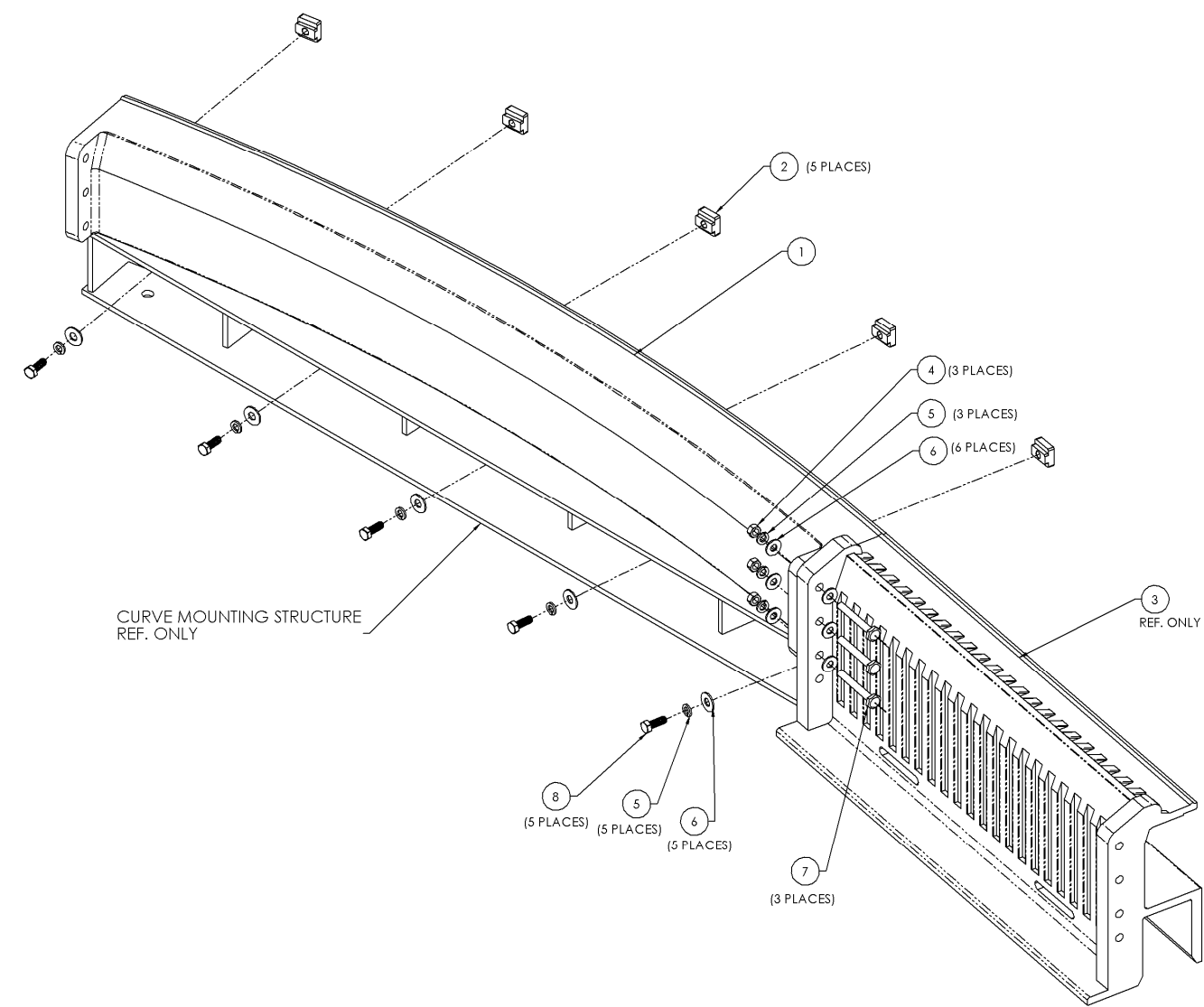
Figure 9-9 Inside Curved Track Assembly
