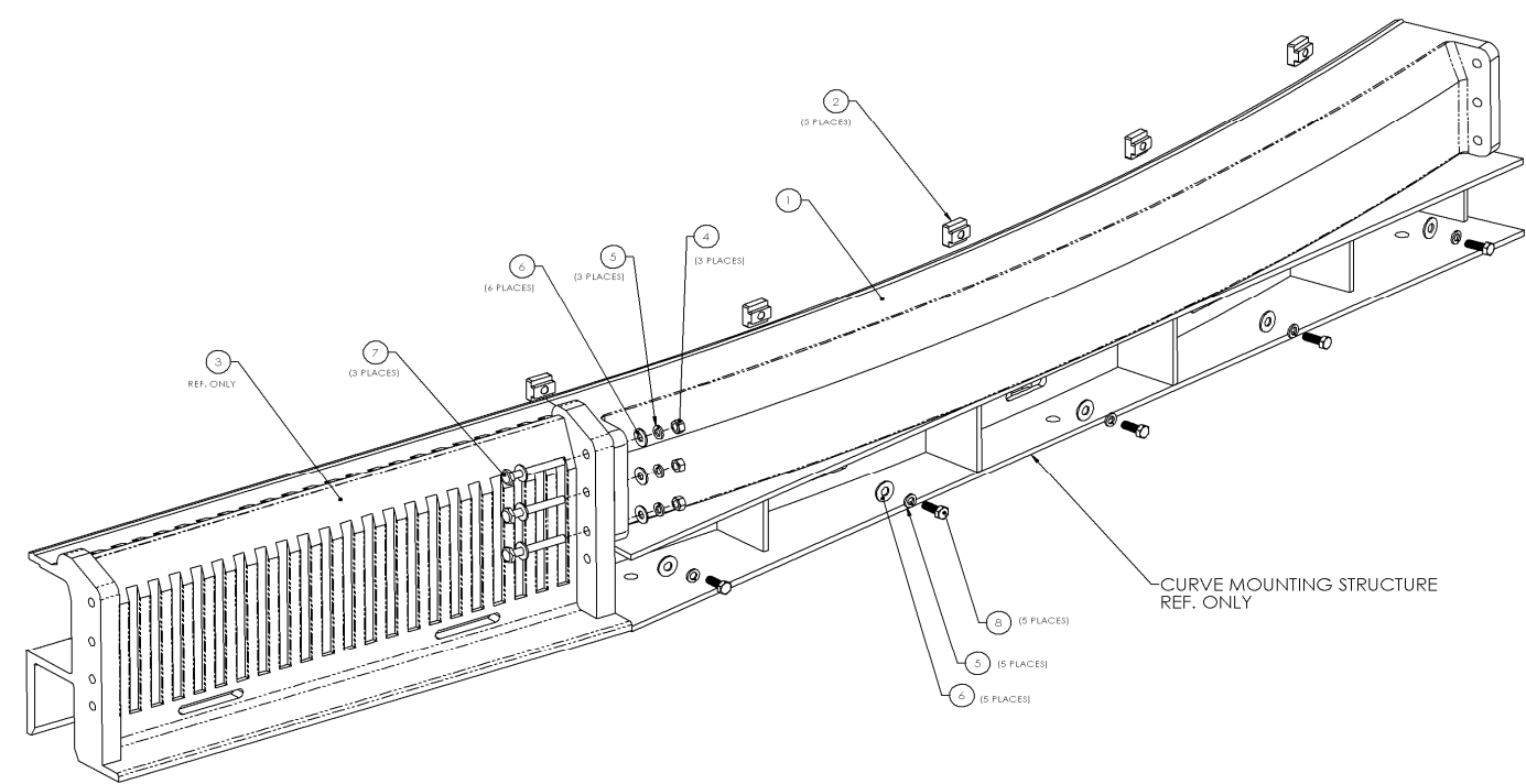
Figure 9-10 Outside Curved Track Assembly
