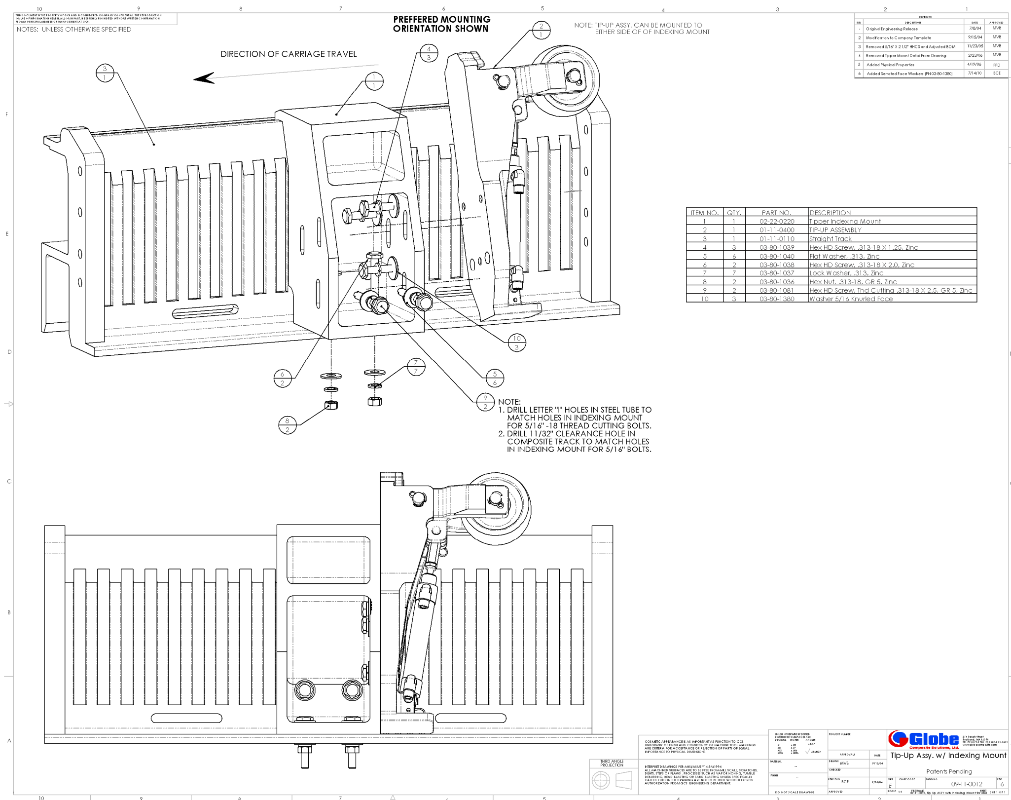
Figure 7.6 Tip-up to Mount & Track Assembly
